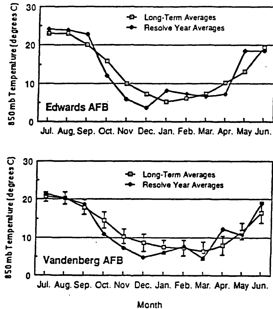
FIGURE 23. Comparison of Long-Term and RESOLVE Year 850 mb Temperatures From the Edwards AFB and Vandenberg AFB Soundings (References 32, 42 and 43). Error bars for Vandenberg AFB are 1 standard deviation of 30-year monthly averages.
