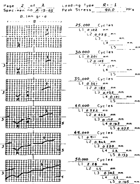
Figure 14.- Example of Data Chart for multi-cracks.
