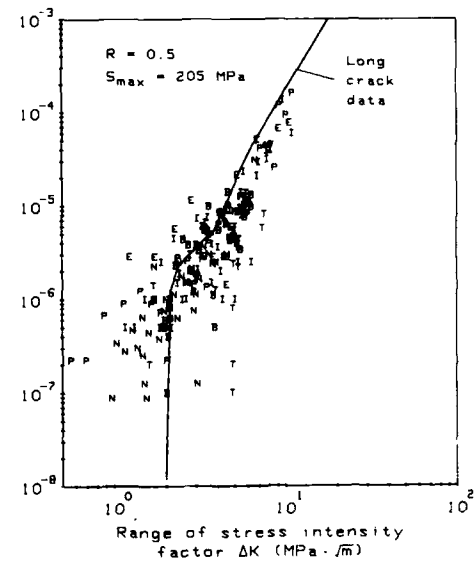
Figure 45.- Constant-amplitude ( R = 0.5 ) results at S_{max} = 205 MPa after "non-interaction" analysis.
