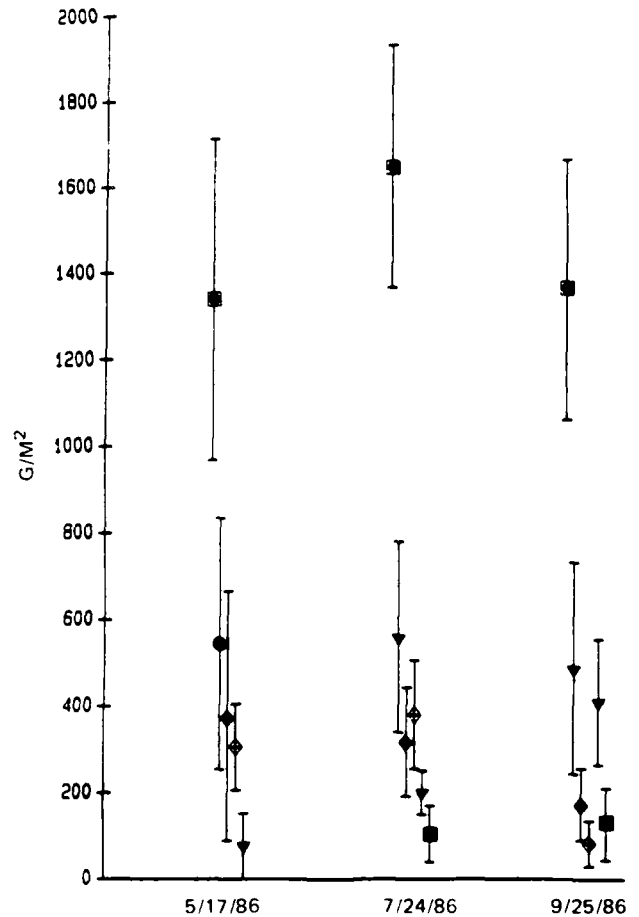
Figure 2. Mean wet weight (spun) of aquatic macrophytes with 95-percent confidence intervals in Devils Lake, Oregon. Symbol interpretation is as follows: Elodea spp. (●), Elodea densa (▼), Elodea canadensis (■), Myriophyllum spicatum (◆), Ceratophyllum demersum (◆), Miscellaneous algae and decayed plant material (▼), and total plant biomass (■)
