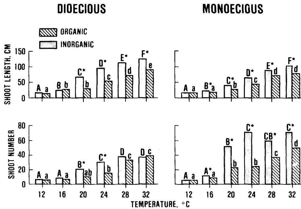
Figure 2. Effects of temperature and sediment type on shoot morphology in dioecious and monoecious Hydrilla . Within each subfigure, shoot lengths or shoot numbers sharing the same letter (uppercase for inorganic sediment and lowercase for organic sediment) do not differ significantly from each other. Asterisks denote significant effects of sediment type on shoot morphology. Duncan's Multiple Range Test was used to determine statistical significance at P < 0.05
