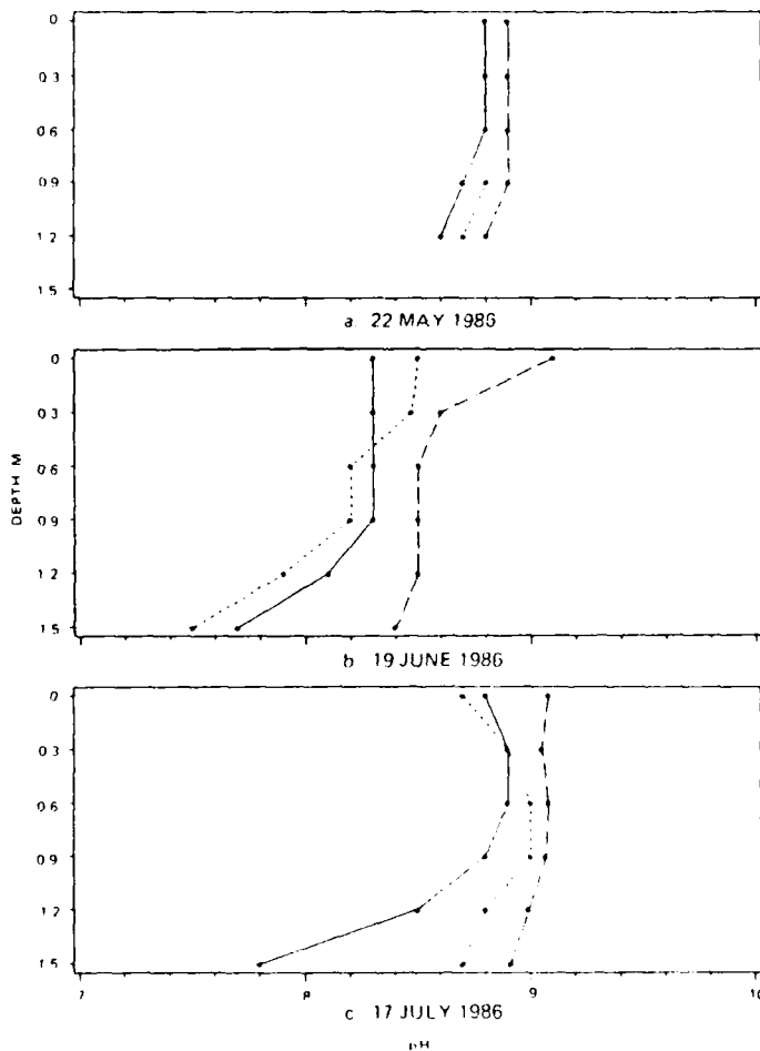
Figure 4. In situ measurements of pH in the southwest bay (Site D) on different dates over a diel cycle (solid line, morning; dotted line, midday; broken line, evening)
