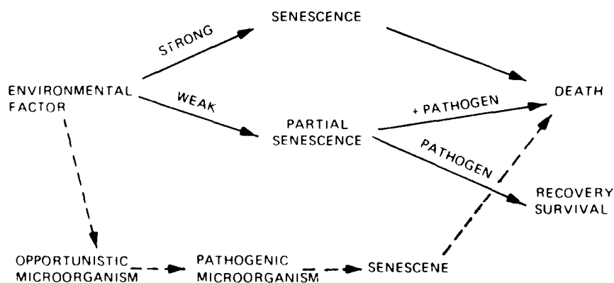
Figure 3. Scheme of interactions between environmentally induced senescence and pathogens
