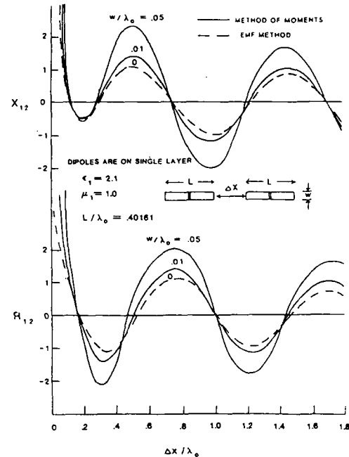
Fig. 5. Mutual impedance versus separation showing a comparison of the moment method solution for two different strip widths and the emf solution for zero strip width.
