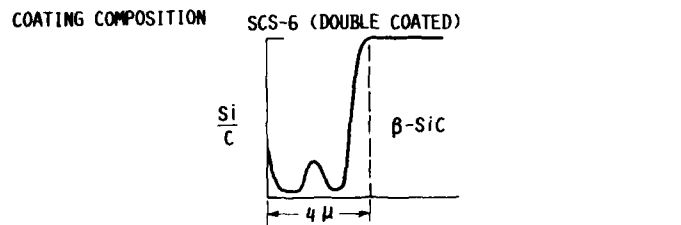
FIGURE 1. - DETAILS OF CVD SiC FIBER.
