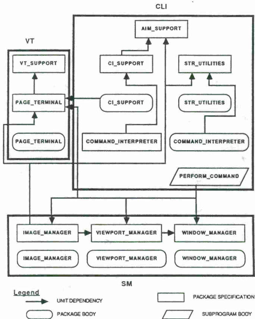
Figure A-1: Evaluation System Model
