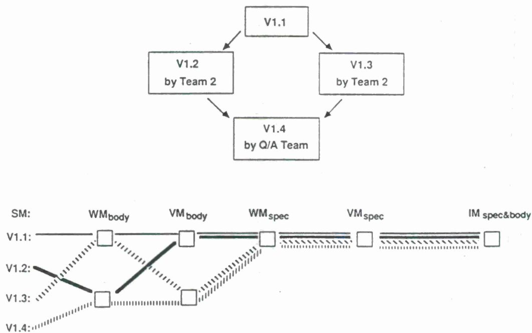
Figure A-5: Version History of SM
