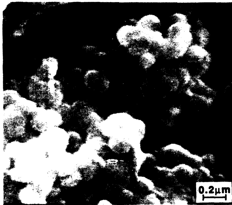
Figure 7. High-magnification SEM micrograph of fracture surface of sample 1430-65.
