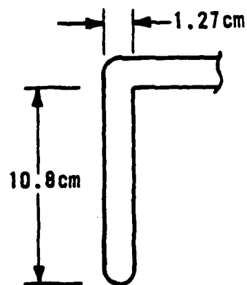
IODINE SOURCE QUARTZ TUBE SIDE VIEW
