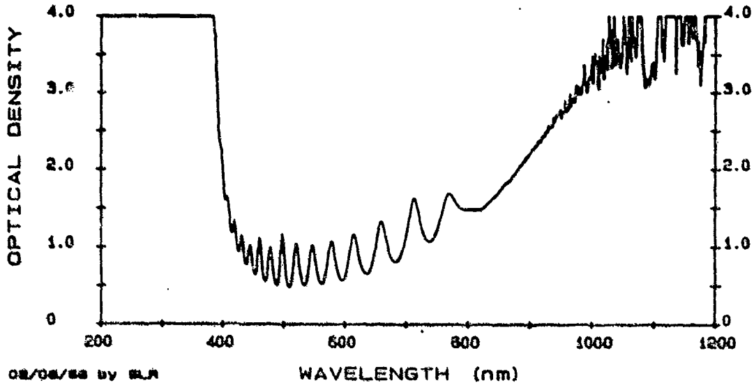
Figure 3A. Open state optical density of PLZT lenses as a function of wavelength.
