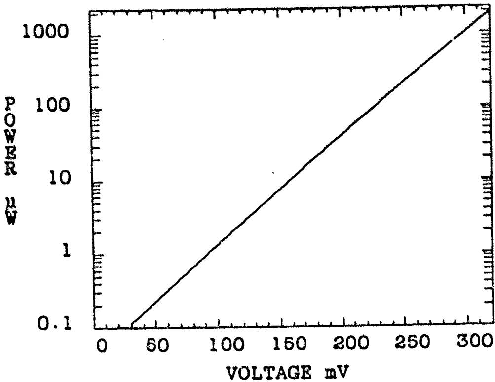
Figure 2A. "Best-fit" function for photodetector calibration curve y(x) = 10^{(-3.96e-6 * x^2 + 1.60e-2 * x - 1.43)}
