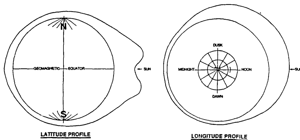
Figure 6. General Ionospheric Layer Shape
