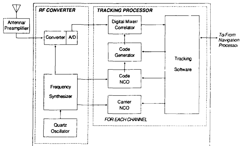
Figure 1. Generic Block Diagram of a GPS Receiver
