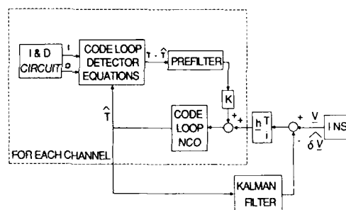
Figure 2. Partitioned Inertial Aiding Scheme (Single Channel)
