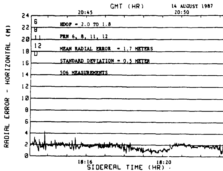
Figure 9. Horizontal Radial Error for U.S. Coast Guard Sea Tests
