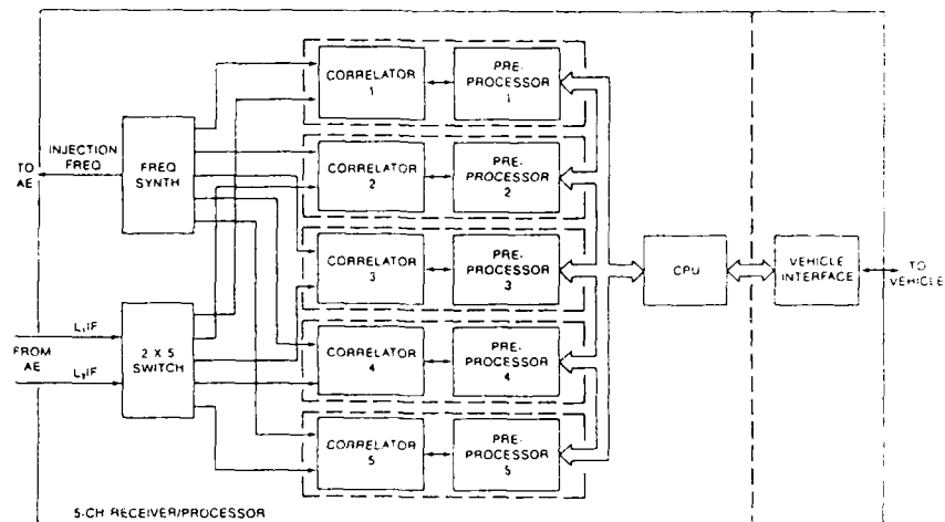
Figure 9. Block Diagram of a Typical 5-Channel GPS Receiver
