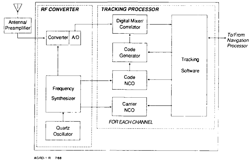
Figure 1. Generic Block Diagram for a GPS Receiver
