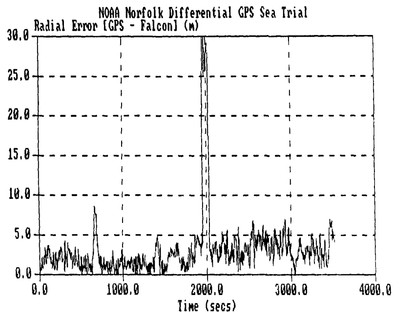
Figure 10. Radial Differential GPS Error During NOAA Sea Test
