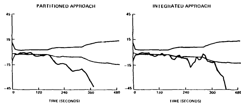
Figure 4. Performance Comparison, Partitioned and Integrated Approaches, for Maximum Jamming Test
