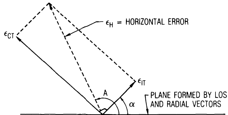
1. Ephemeris Error Geometry
