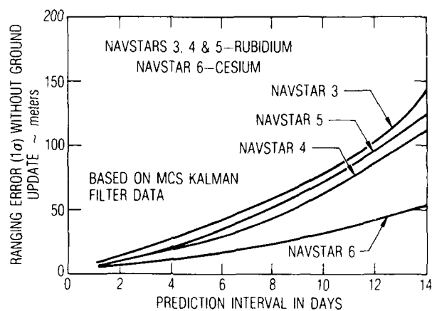
10. Clock Prediction Error
