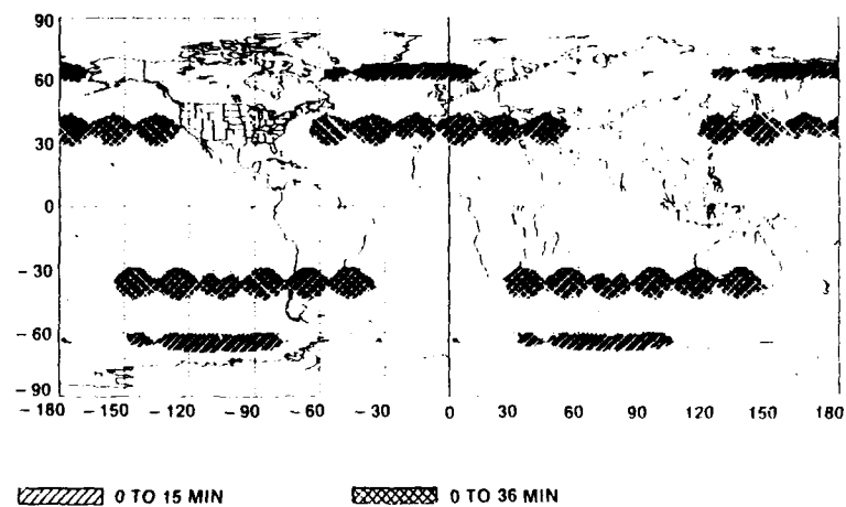
Figure 3. Areas of Degraded Performance where PDOP > 10 (mask angle = 5°)
