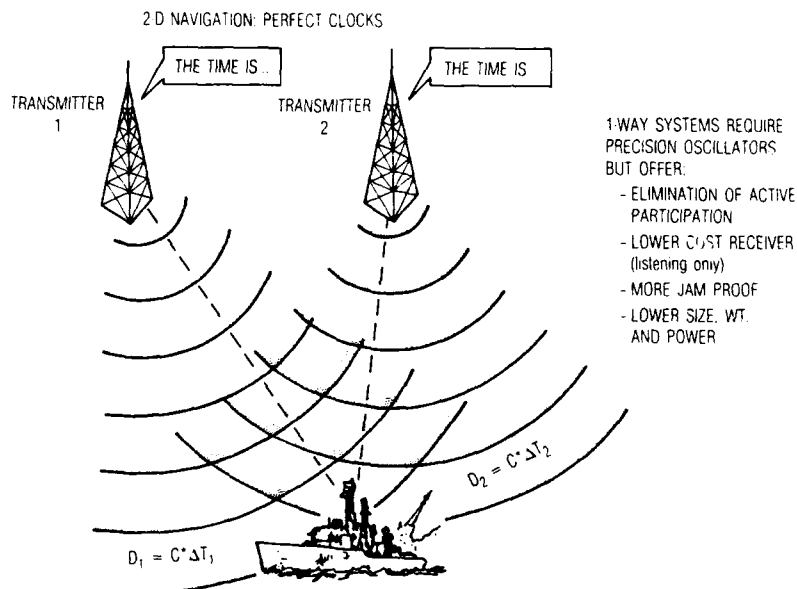
Figure 2. Electronic One-Way Ranging System
