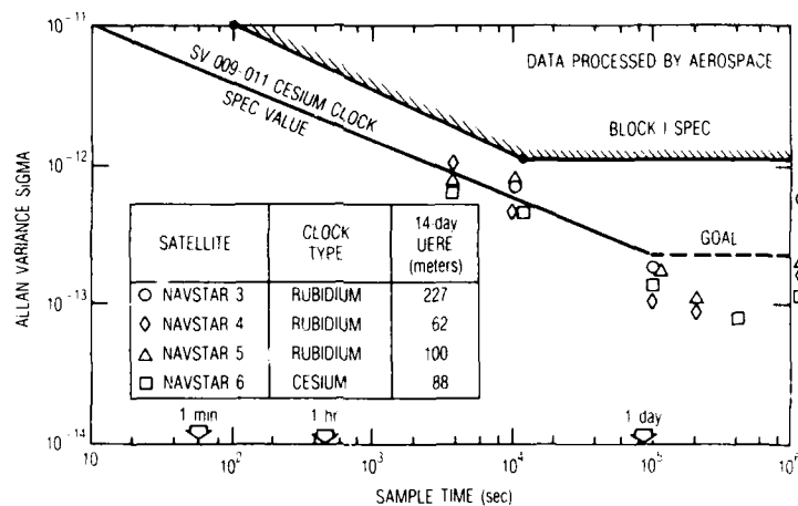
9. Frequency Standard On-Orbit Performance
