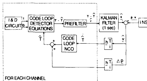
Figure 3. Integrated Inertial Aiding Scheme (Single Channel)
