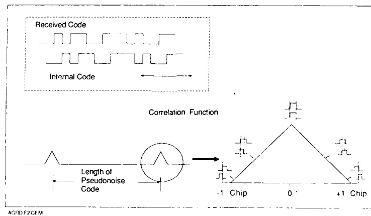
Figure 2 Code Loop Correlation Process
