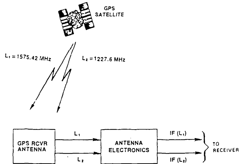
Figure 4. Simplified Functional Diagram of GPS Antenna Subsystem
