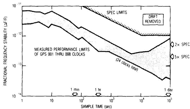
8. Frequency Standard Stability Performance
