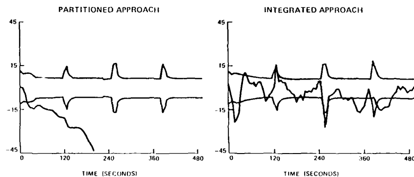
Figure 5. Performance Comparison, Partitioned and Integrated Approaches, for Maximum Jamming and Dynamics Test
