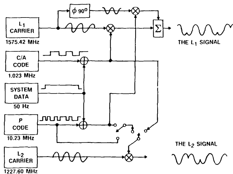
Figure 2. Satellite Signal Modulation
