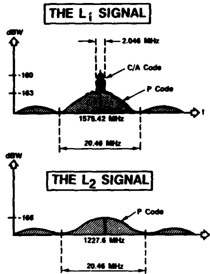
Figure 3. GPS Signal Frequency Spectrum
