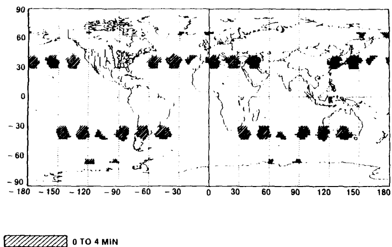
Figure 4. Areas of Degraded Performance where PDOP > 50 (mask angle = 5°)
