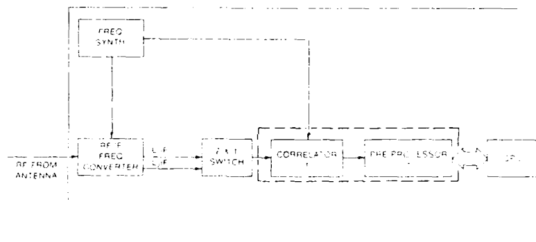
Figure 10. Block Diagram of a Typical 1-Channel GPS Receiver
