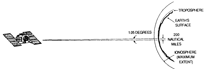
Figure 3. Relative Geometry in Typical Differential GPS Application
