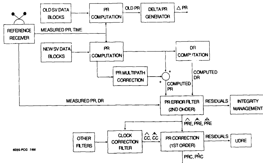
Figure 5. Pseudorange Error Estimation Process in the Reference Station
