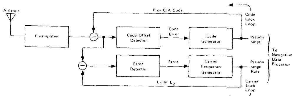
Figure 12. Generic Receiver Operation Block Diagram
