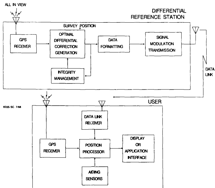
Figure 1. Differential GPS Concept
