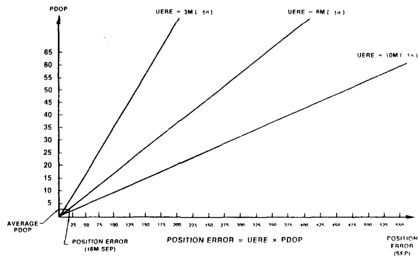
Figure 2. PDOP, Range Accuracy and Position Accuracy Relations
