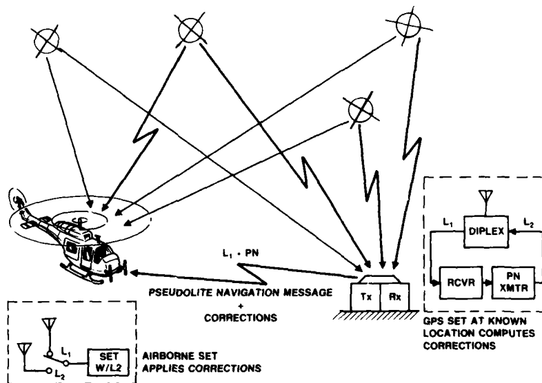
4. Differential GPS with Pseudolite
