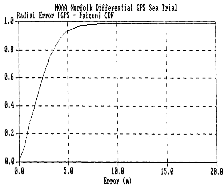
Figure 11. Cumulative Distribution of Radial Errors for NOAA Test
