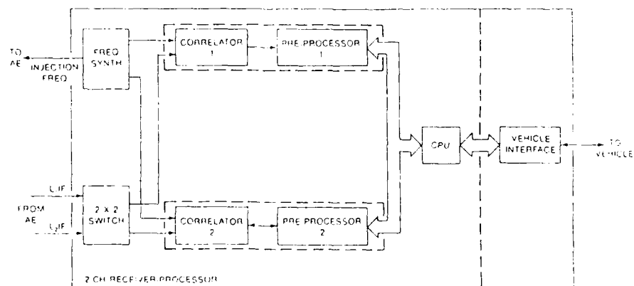
Figure 11. Block Diagram of a Typical 2-Channel GPS Receiver
