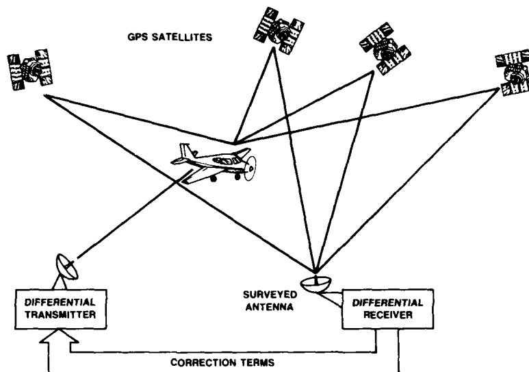
3. Differential GPS Operation
