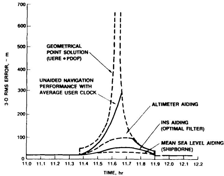
Figure 5. GPS Receiver Performance during a Period of Degraded Performance when Aided
