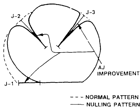
Figure 8. CRPA-Adaptive Array Antenna Performance Pattern
