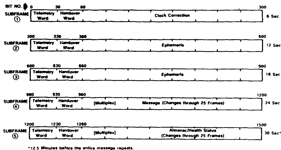
Figure 1. The Navigation Message
