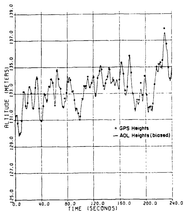
Figure 12. P-3 Kinematic Phase Tracking Performance
