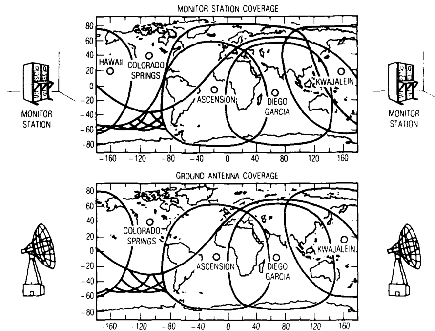
5. Ground Segment Coverage
