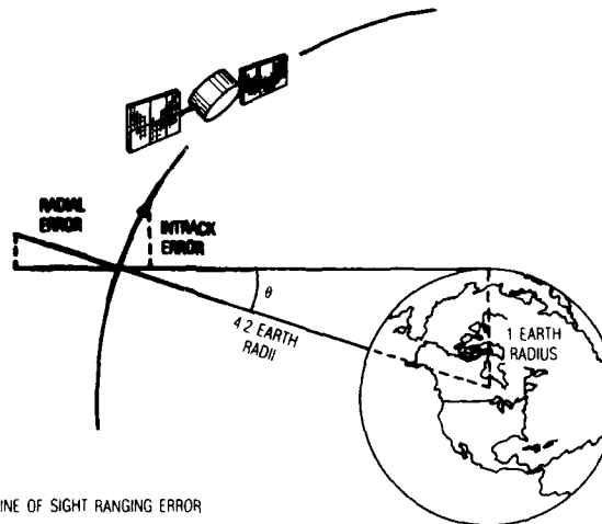
1. Ephemeris Error Geometry
