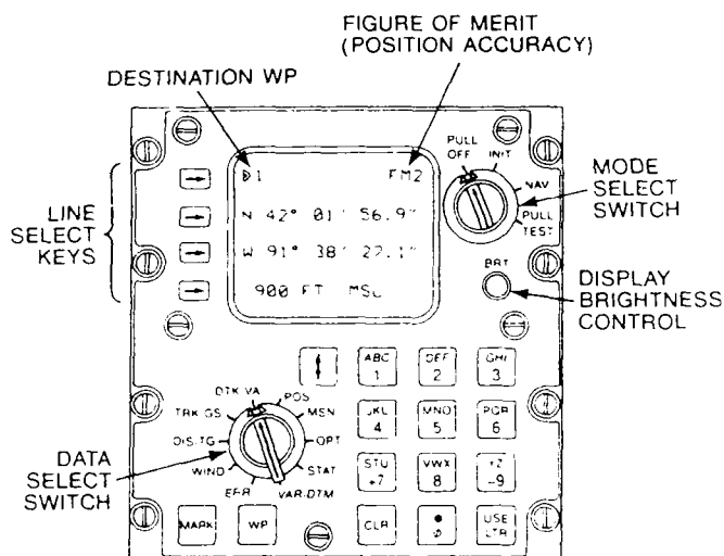
Figure 2. Typical Control Display Unit for Aircraft/Shipboard Applications
