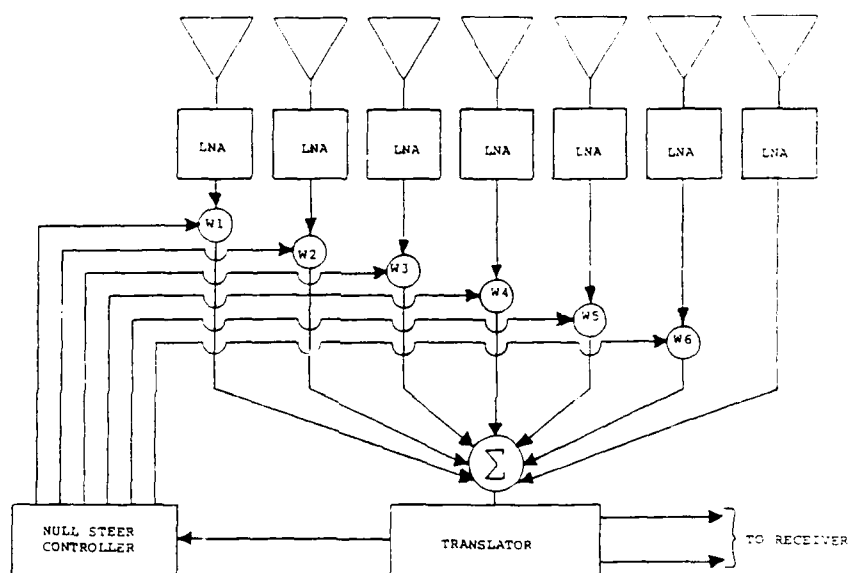
Figure 7. Functional Block Diagram of Null Steering Process for a 7-Element Antenna
