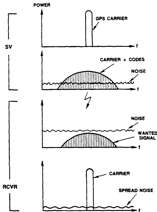
Figure 4. Spread Spectrum Used in GPS
