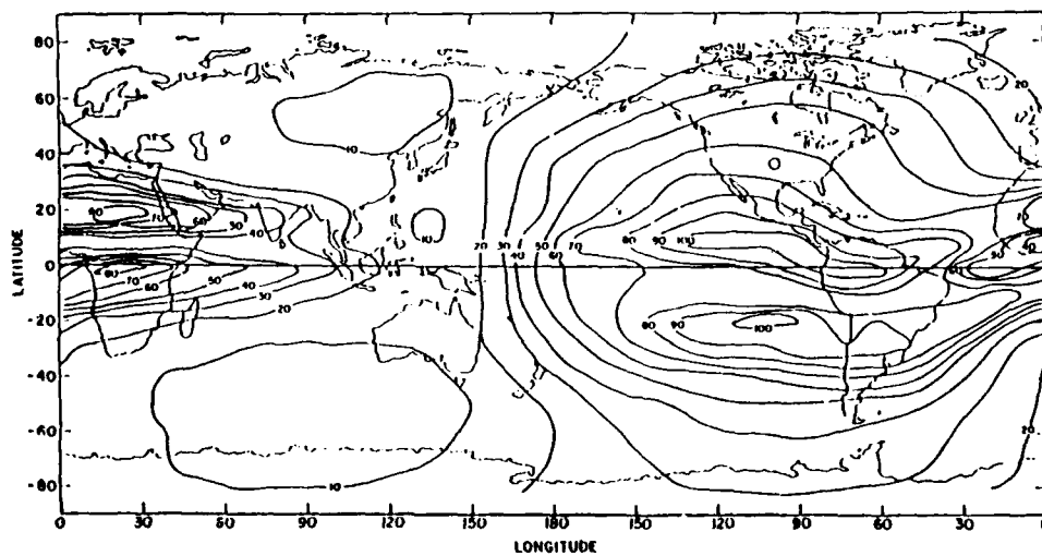
CONTOURS OF VERTICAL TEC, IN UNITS OF 10^{16} EL/M 2 COLUMN, FOR 2000 UT, MARCH 1980.
