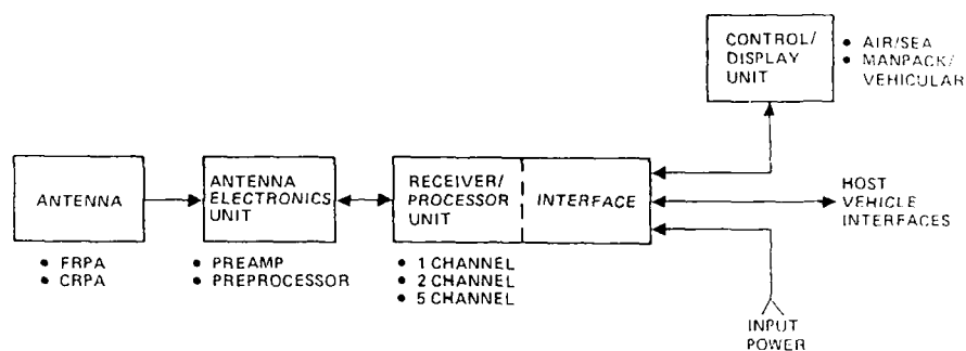
Figure 1. Description of a Typical GPS User Equipment Set
