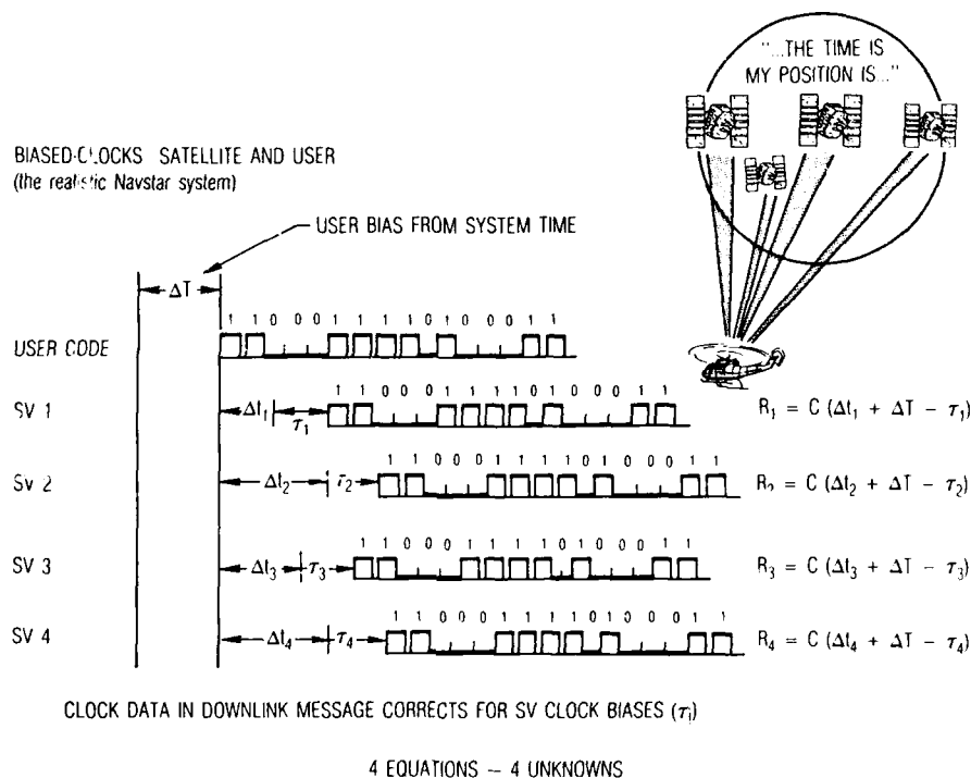
Figure 5. Clock and Ephemeris Parameters
