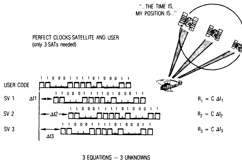
Figure 3. Spaceborne One-Way Ranging
