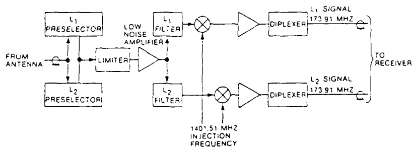
Figure 6. Functional Diagram of Antenna Electronics for FRPA
