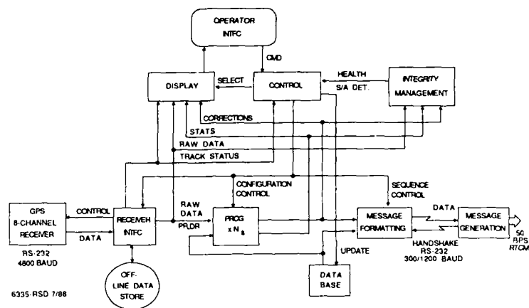
Figure 4. Differential GPS Reference Station Functional Design
