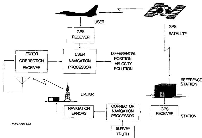
Figure 1. Differential GPS Concept
