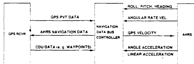
Figure 7. GPS/AHRS Integration
