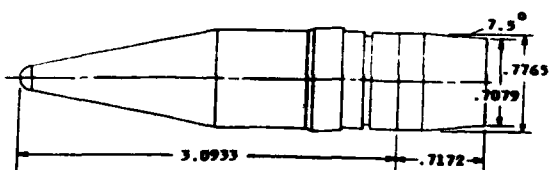
c. Boattail Configuration
