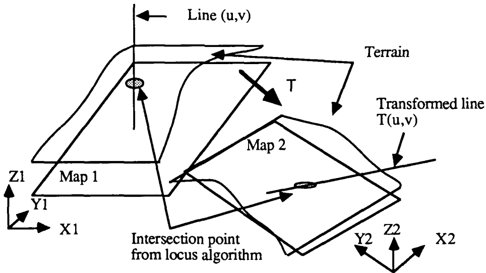
Figure 37: Principle of the iconic matching algorithm
