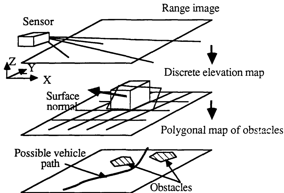
Figure 15: Building the obstacle map
