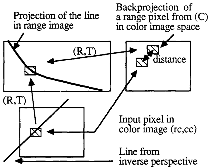
Figure 42: Geometry of the "video \rightarrow range" transformation
