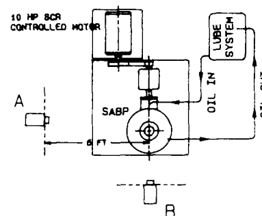
c) AIRBORNE NOISE SET-UP
