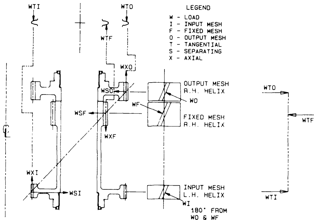
FIGURE 8 - IDENTIFICATION OF SABP GEAR TOOTH LOADS
