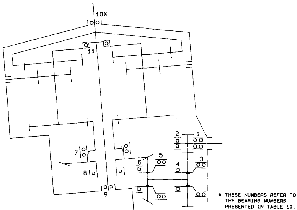
FIGURE 16 - BEARING ARRANGEMENT
