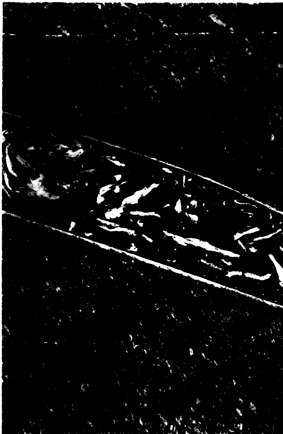
Fig. 23 Projectile indentation (# 925): detail of broken shear band with fragments of transformed material
