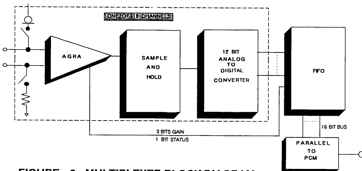
FIGURE 2. MULTIPLEXER BLOCK DIAGRAM.
