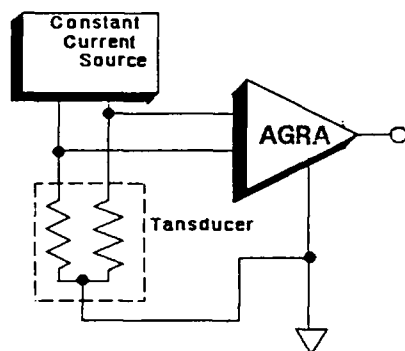
FIGURE 1. CONSTANT CURRENT EXCITATION.
