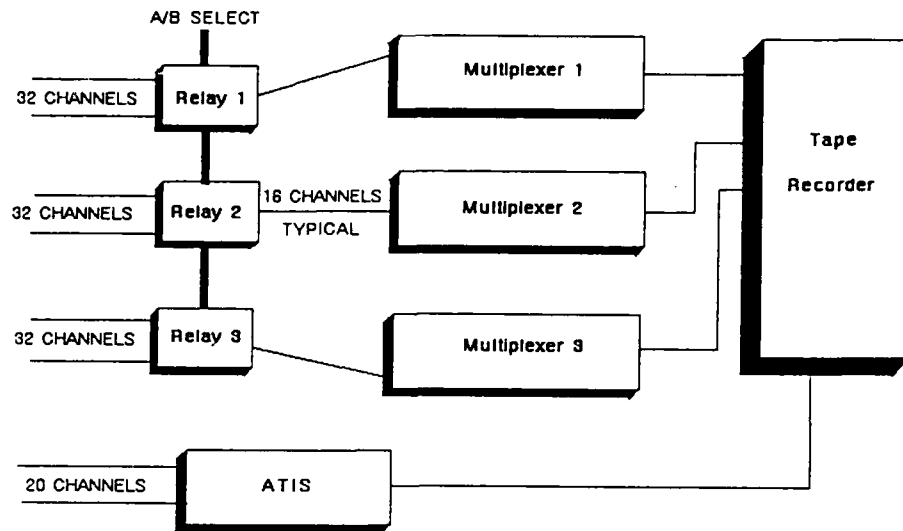
FIGURE 3. A-10 SYSTEM BLOCK DIAGRAM.
