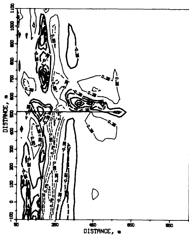
Figure A12. 3 September to 5 December 1986 change diagram
