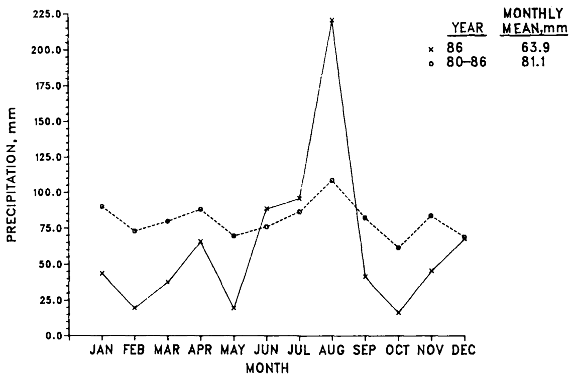
Figure 8. Mean monthly precipitation
