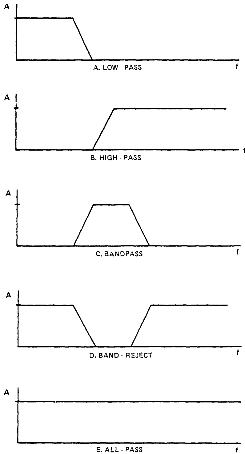
FIGURE 1. COMMON FILTER AMPLITUDE FUNCTIONS
