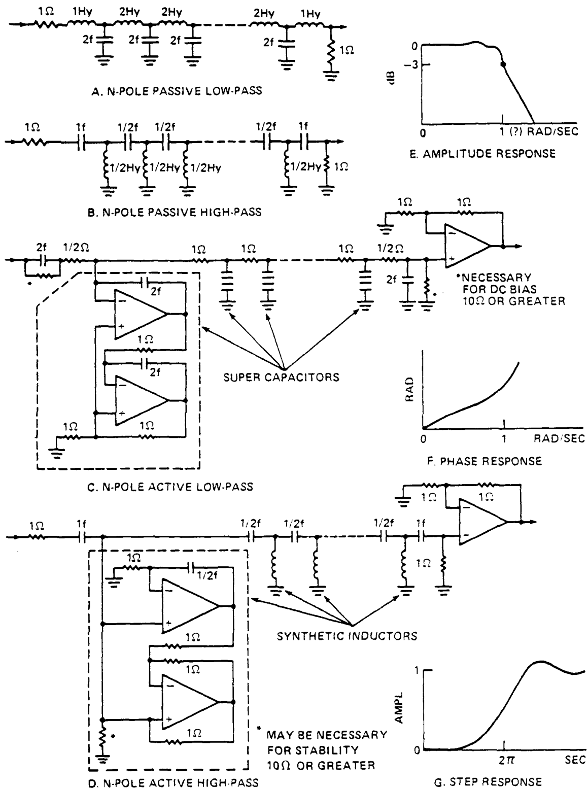
FIGURE 12. CONSTANT-K FILTERS
