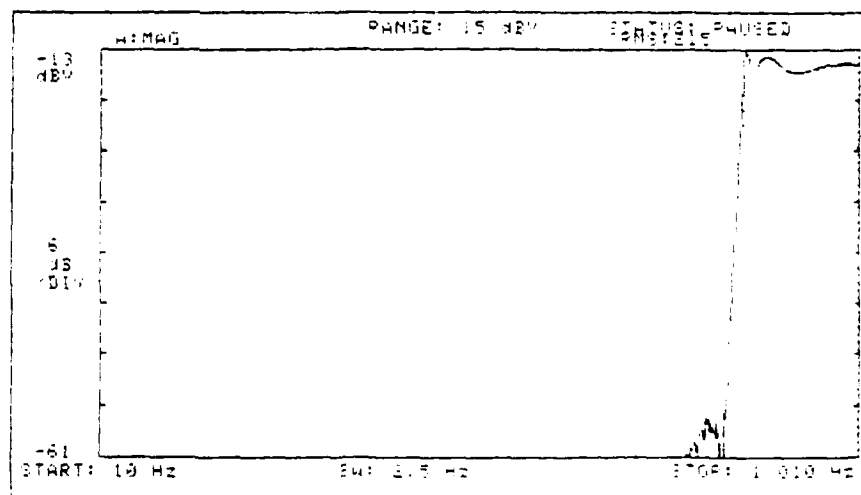
FIGURE A-31. SWITCHED-CAPACITOR ELLIPTIC RESPONSE
