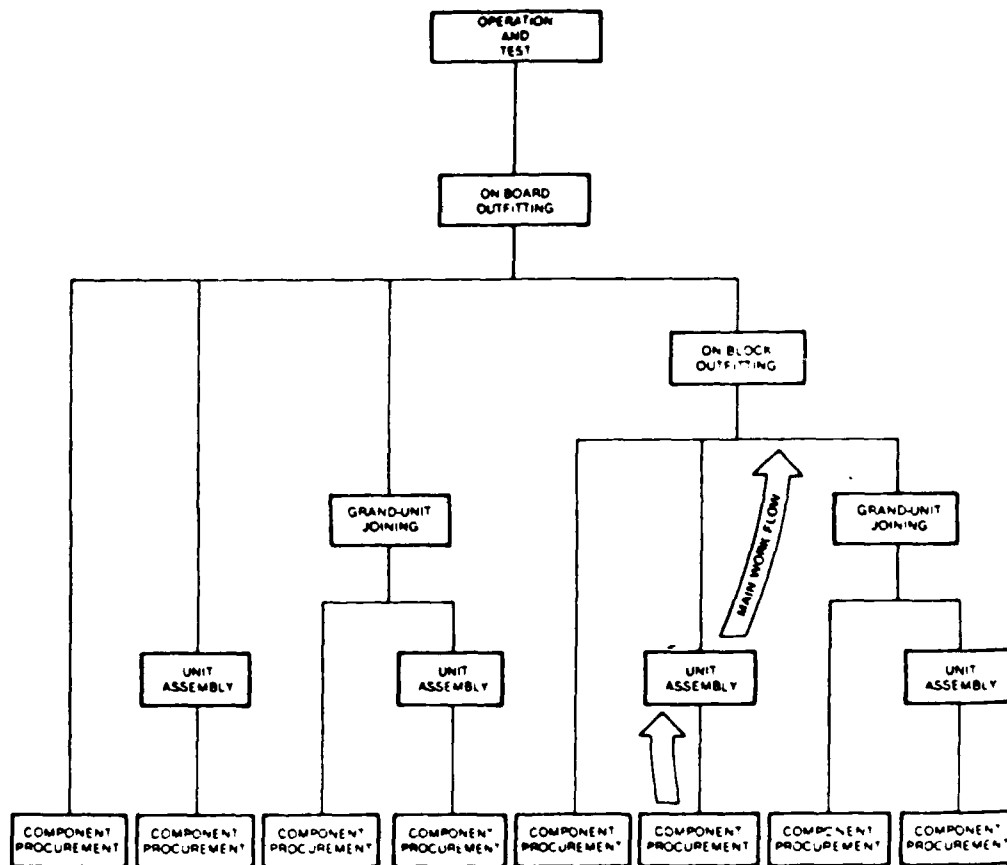
Figure 2-8. Manufacturing Levels for ZOFG.(50)
