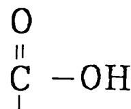
OXALATE
