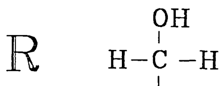
GLYCOLATE
