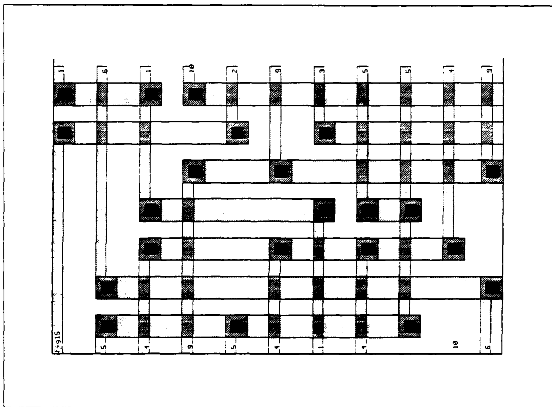
Figure 16: A channel unroutable by the greedy algorithm.
