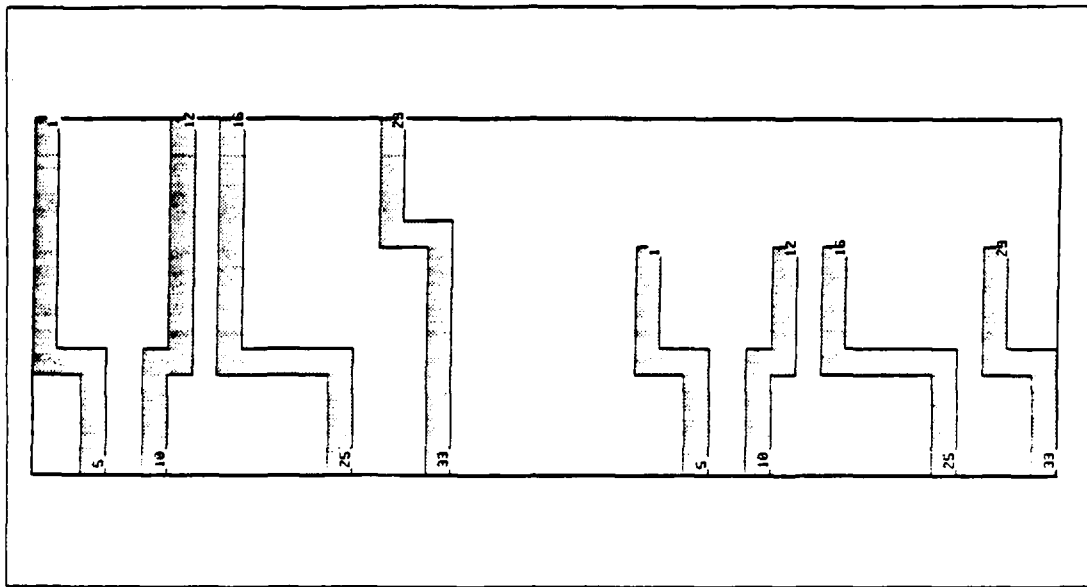
Figure 23: Solution to river routing problem. (a) MacPitts solution. (b) optimal solution.
