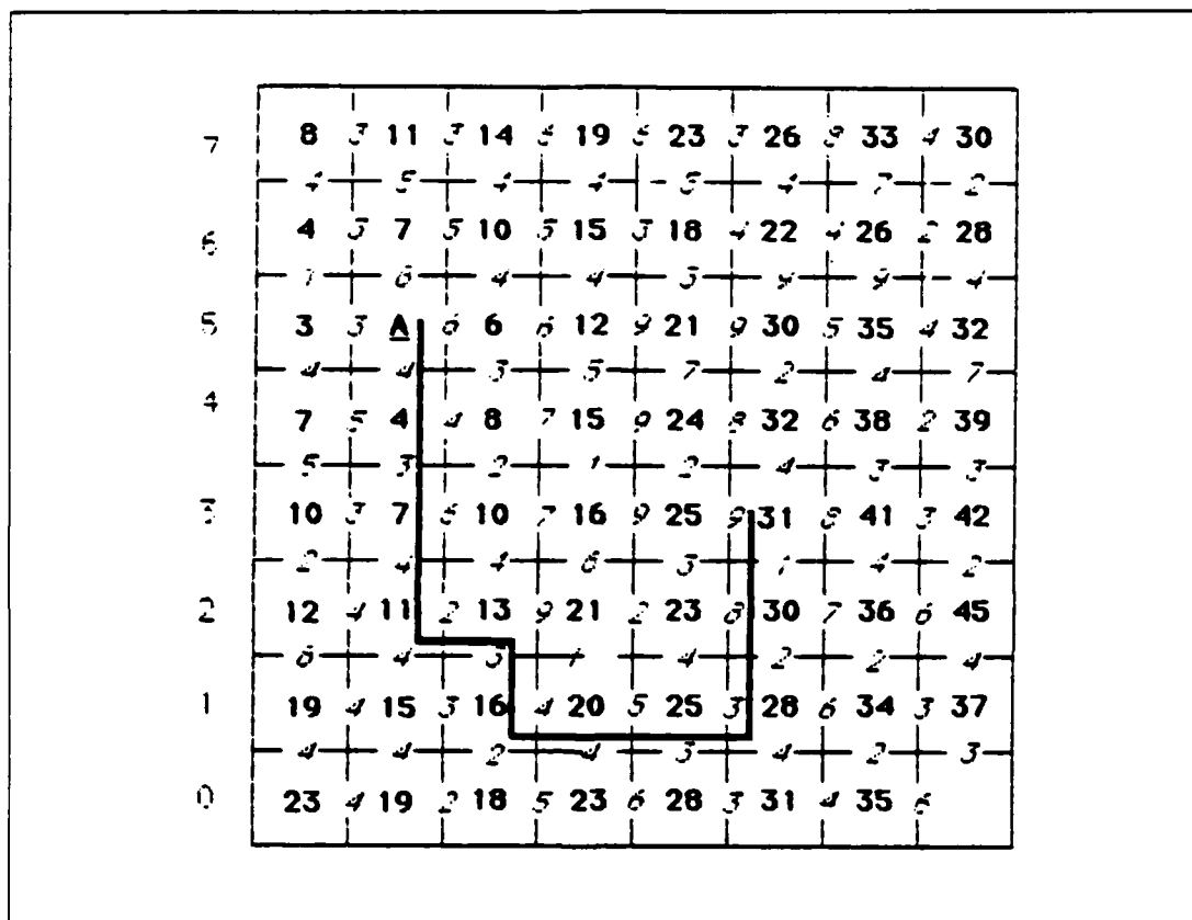
Figure 10: The backtrace route.
