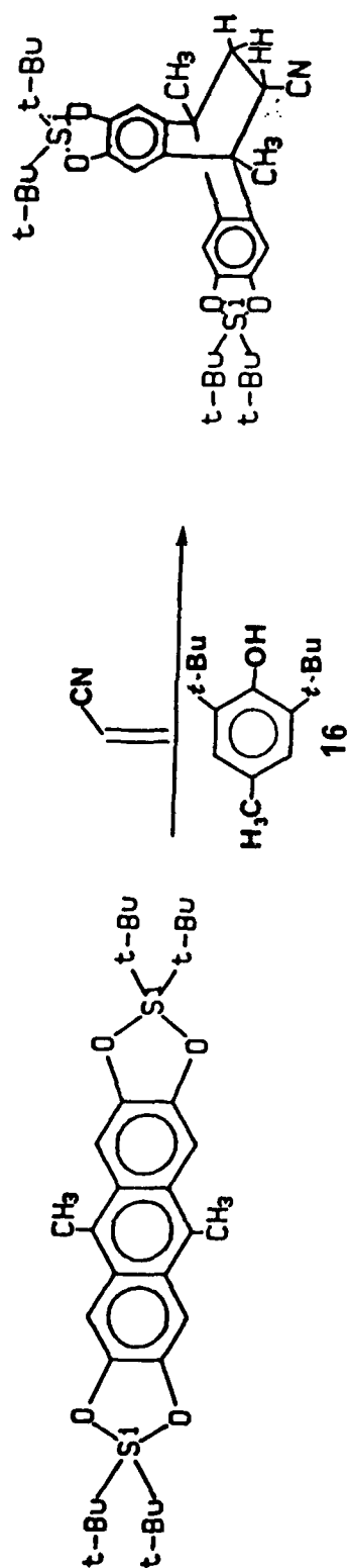
FIGURE 11 : Synthesis of bis-(di-t-butylsiladioxy)[b,1]-9,10-dimethyl-11-cyanoethanoanthracene.
