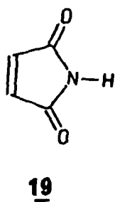
FIGURE 17 : Dienophiles used in Diels-Alder kinetic studies.
