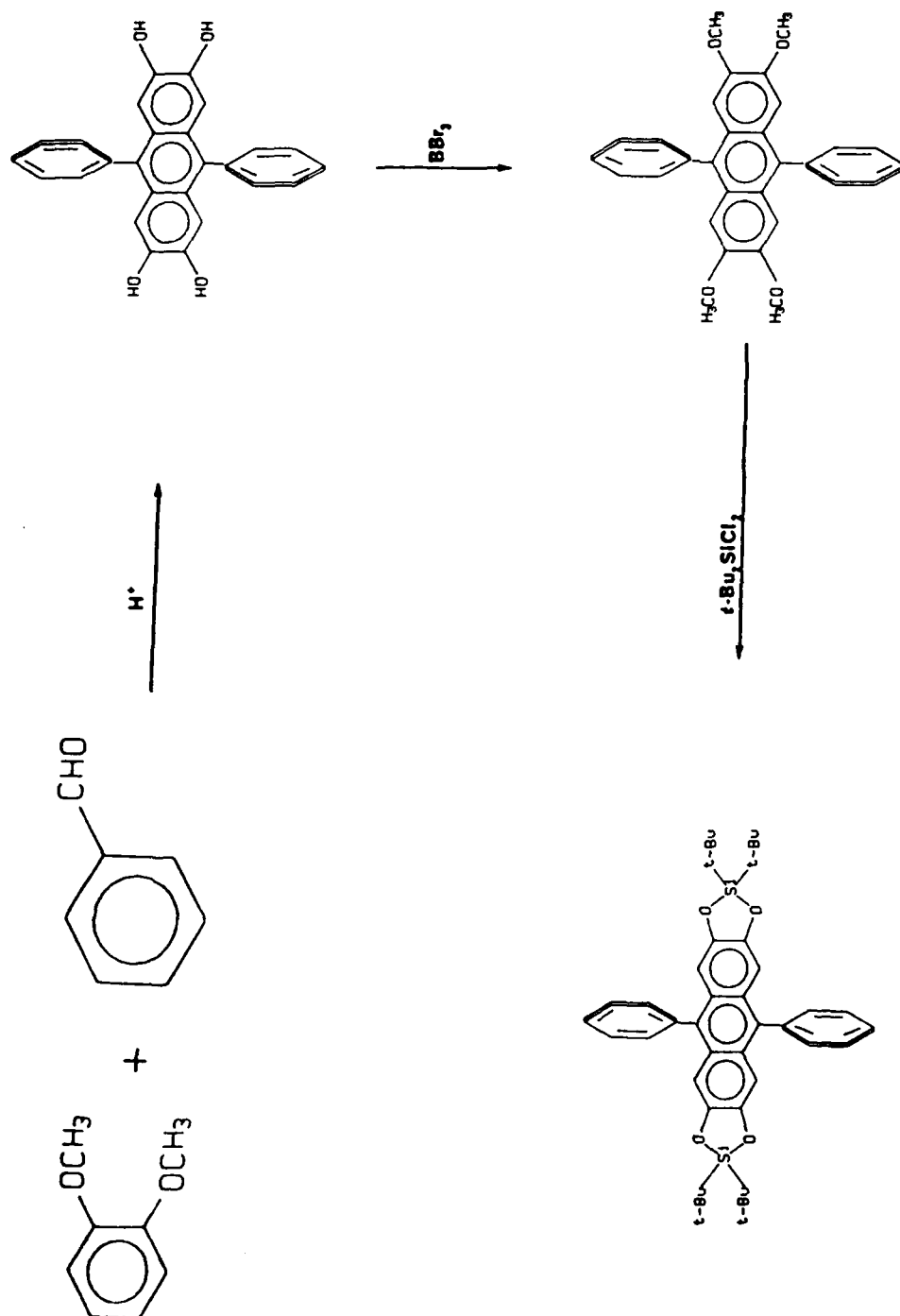
FIGURE 13 : Synthesis of bis-(di-t-butylsiladioxy)[b,1]-9,10-diphenylanthracene.
