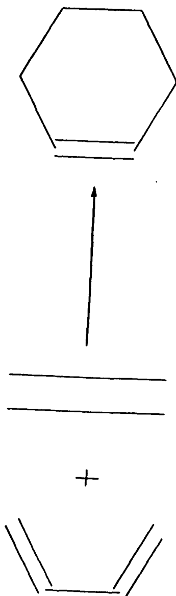
FIGURE 3 : Diels-Alder reaction scheme (general).
