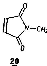
FIGURE 17 : Dienophiles used in Diels-Alder kinetic studies.
