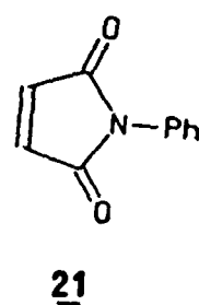
FIGURE 17 : Dienophiles used in Diels-Alder kinetic studies.
