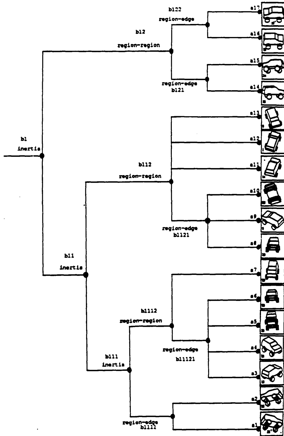
Figure 3: Interpretation tree for a toy wagon
