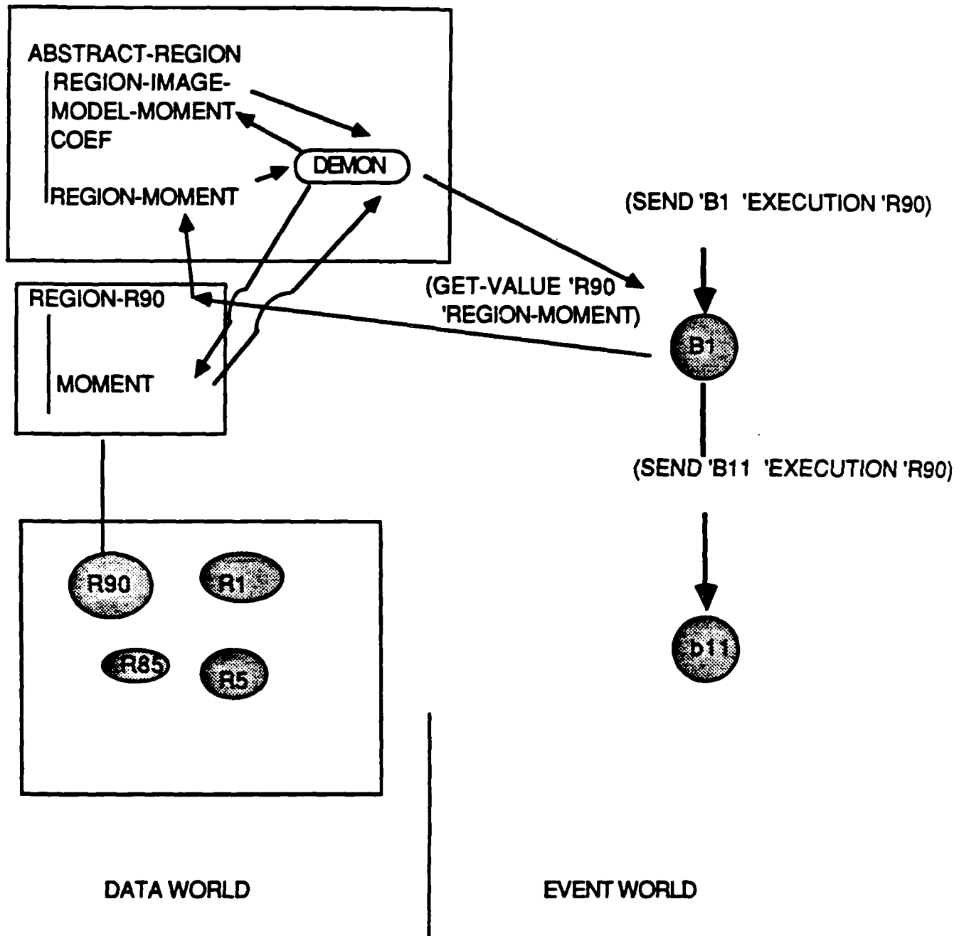
Figure 9: Retrieving feature value from a region.
