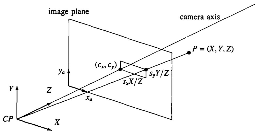
Figure 2: Camera model
