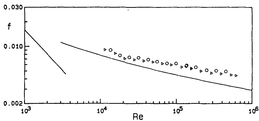
c) B-3 ( L/d_o = 8 )
