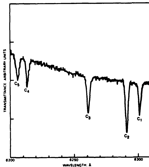
Figure 5. Absorption spectrum of |2H|11/2 manifold of \text{Nd}^{3+} superimposed on first strong \text{Cr}^{3+} band, recorded at liquid helium temperature.
