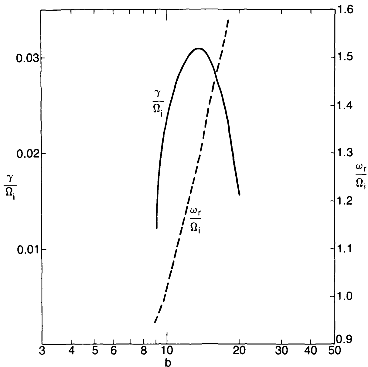
Fig. 10 — A plot similar to the figure (9). Here u = 0.038 and rest of the parameters are identical to figure (3).
