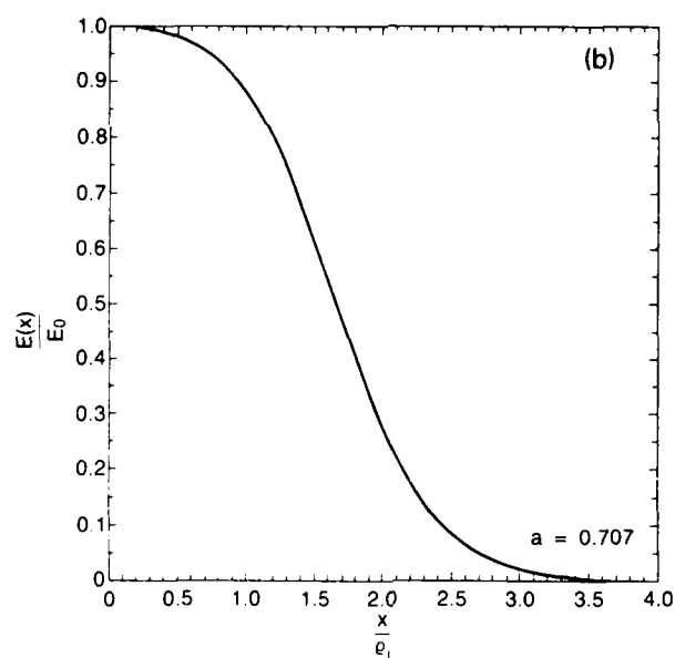
Fig. 7 — The transition from a sharp to a smooth profile given in the equation (39). Here \epsilon = 0.3 , and (a) a = 0.1 and (b) a = 0.707 .
