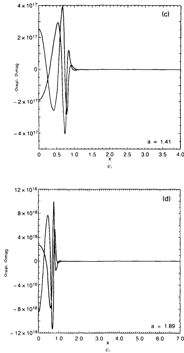
Fig. 8 (Continued) — The real and imaginary parts of the corresponding eigenfunctions for the profiles in figure (7). Here b = 8 , \mu = 1837 , V_E = 0.6 , \tau = 3.5 , u = 0.011 and \epsilon_n = -0.07 if x_{n0} - 0.9_{\rho i} < x < x_{n0} + 0.9_{\rho i} and x_{no} = 1.66_{\rho i} . (c) a = 1.41 and (d) a = 1.89 .
