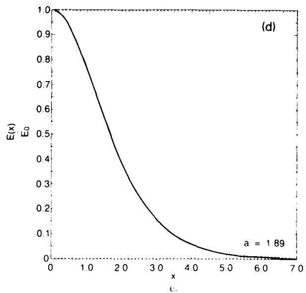
Fig. 7 (Continued) — The transition from a sharp to a smooth profile given in the equation (39). Here \epsilon = 0.3 , and (c) a = 1.41 and (d) a = 1.89 .
