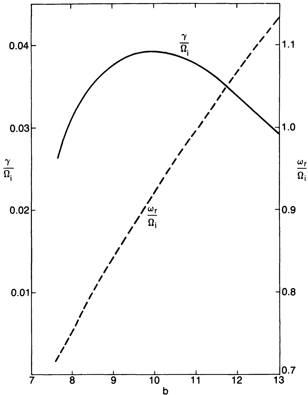
Fig. 9 — A plot of the normalized real and imaginary parts of the eigenfrequency of the ion-cyclotron-like instability against b . Here \epsilon = 0.3 , u = 0.011 , a = 1.87 , \tau = 3.5 , V_E = 0.6 , \mu = 1837 and \epsilon_n = -0.07 if x_{n0} - 0.9\rho_i < x < x_{n0} + 0.9\rho_i and zero otherwise and x_{n0} = 1.66\rho_i .
