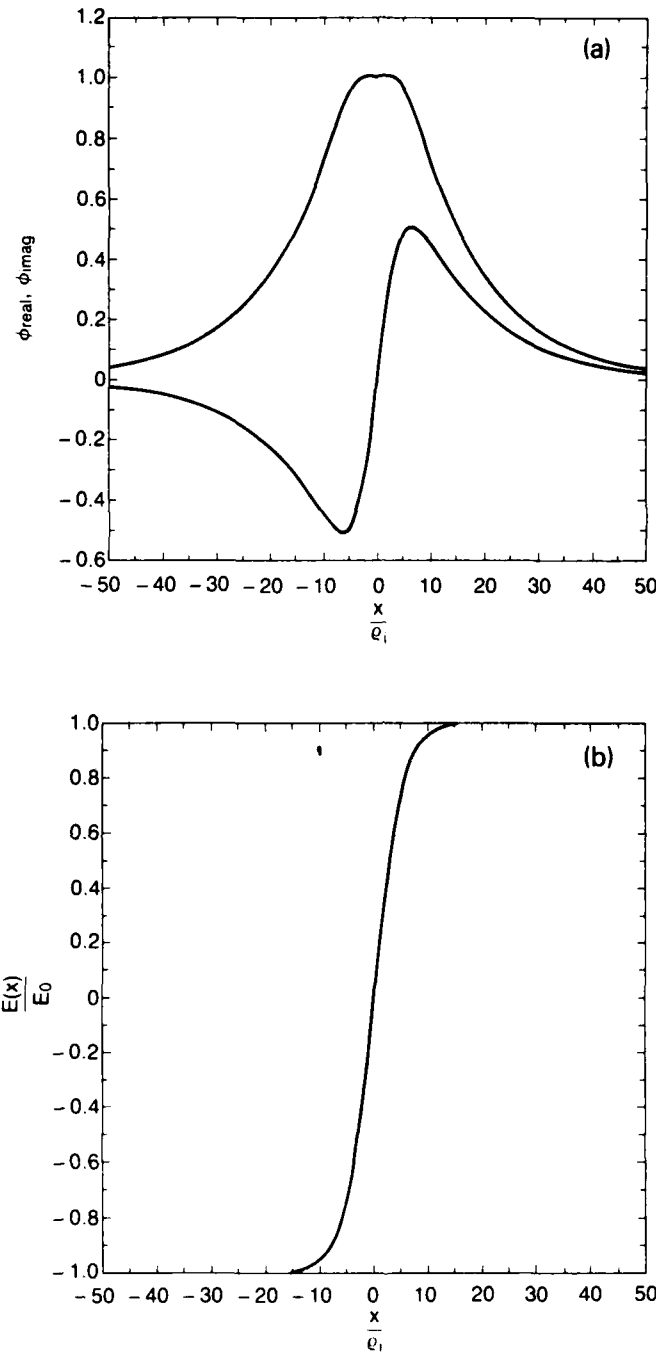
Fig. 1 — (a) Real and imaginary parts of a typical eigenfunction for E = E_0 \tanh(x/L) profile. Here \epsilon = 0.19 , k_y \rho_i = 0.074 , V_E = 0.764 , \mu = 1837 , u = 0.0001 and \tau = 1 . (b) The external electric field profile for \epsilon = 0.19 .
