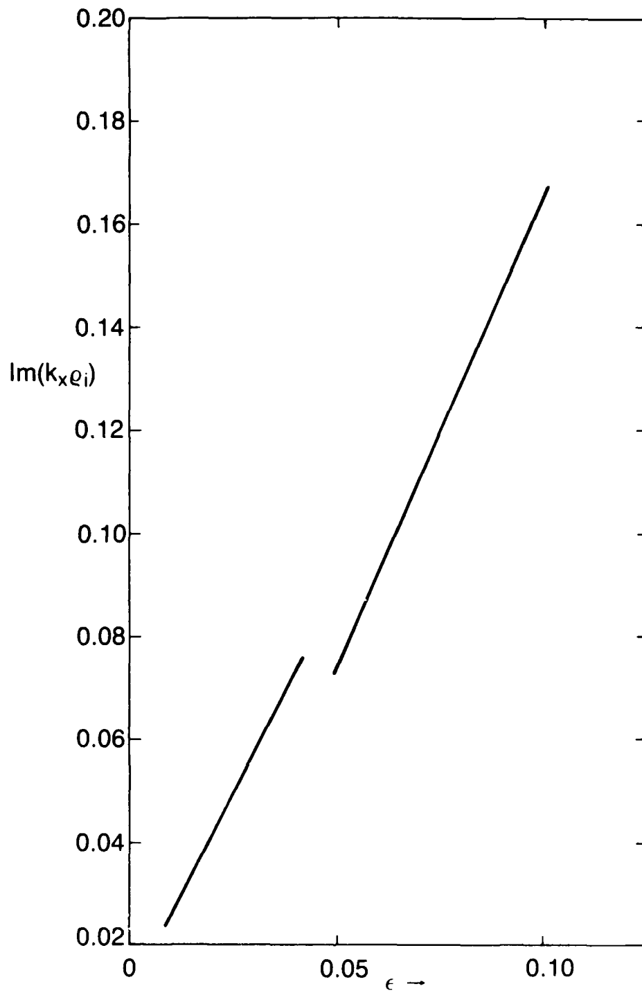
Fig. 6 — A plot of the \text{Im}(k_x \rho_i) against \epsilon . The linear dependence confirms the scaling \gamma/V_G \propto 1/L . Here V_E = 2.9 , \tau = 1 , u = 0.0001 and \mu = 1837 .
