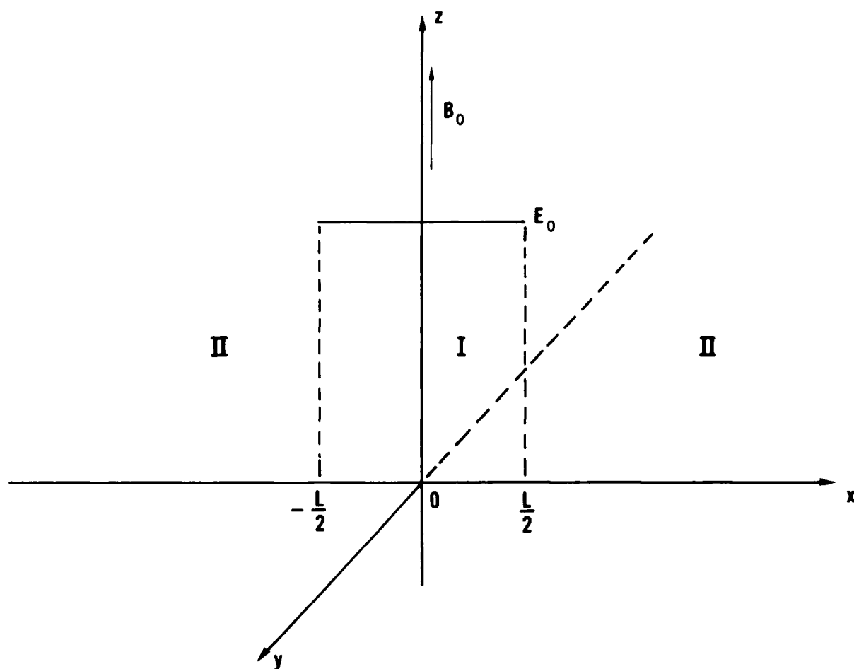
Fig. 5 — A schematic representation of the piecewise continuous d.c. electric field profile.
