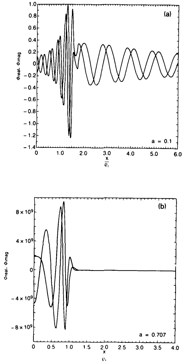
Fig. 8 — The real and imaginary parts of the corresponding eigenfunctions for the profiles in figure (7). Here b = 8 , \mu = 1837 , V_E = 0.6 , \tau = 3.5 , u = 0.011 and \epsilon_n = -0.07 if x_{n0} - 0.9\rho_i < x < x_{n0} + 0.9\rho_i and x_{n0} = 1.66\rho_i . (a) a = 0.1 and (b) a = 0.707 .
