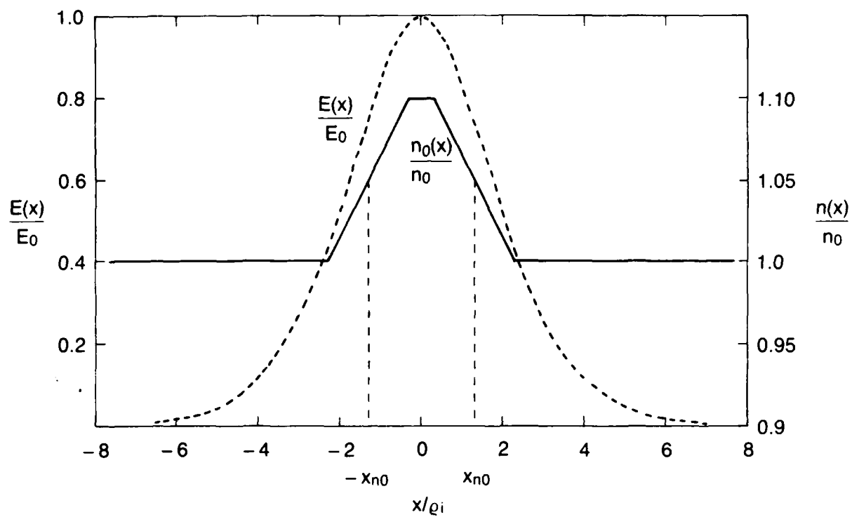
Fig. 4 — The equilibrium field and density configuration used in the calculations of figure (3). Here x_{n0} = 1.33\rho_i \epsilon_n = -0.05 when x_{n0} - \rho_i < x < x_{n0} + \rho_i and zero otherwise.
