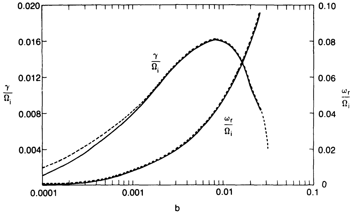
Fig. 2 — The real and imaginary frequencies normalized by \Omega_i for the K-H instabilities for the d.c. electric field profile given by E = E_0 \text{sech}^2(x/L) are plotted as a function of b . The solid lines are the eigenvalues of the equation (29) while the dotted lines are the fluid results given in the reference (9). Here \epsilon = 0.1 , \tau = 1 , \mu = 1837 and u = 0.0001 .
