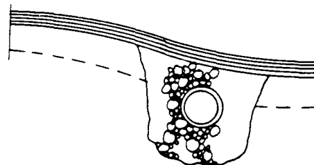
(d) Culvert carries water under driveway
