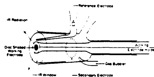
SCHEMATIC DIAGRAM OF ELECTROCHEMICAL INFRARED CELL
