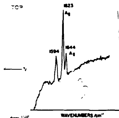
mM pyrene in acetonitrile. The limits of the modulation potential were set between +0.5 and -1.2 V vs Ag/Ag + where no electrochemical reaction was occurring. Therefore, the bands appearing in the difference spectra are due to the changing electric field rather than a chemical process. The band which occurs at ~1640 cm -1 corresponds to the totally symmetric ( A_g ) C-C stretching mode of pyrene. The Raman spectrum of pyrene was obtained in our labs and three bands were found in this frequency region (Fig. 3): The
