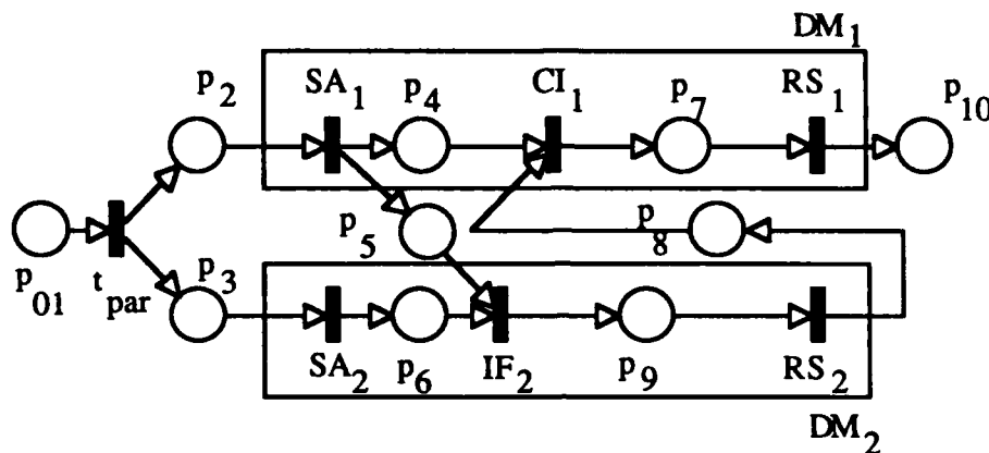
Fig. 5.1 Two-Person Hierarchical Organization
