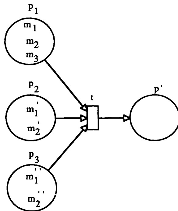
Fig. 3.8 Token Selection
