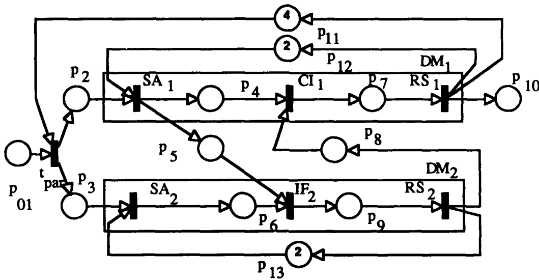
Fig.5.3 (a) Example1, Case 2 - Initial Marking
