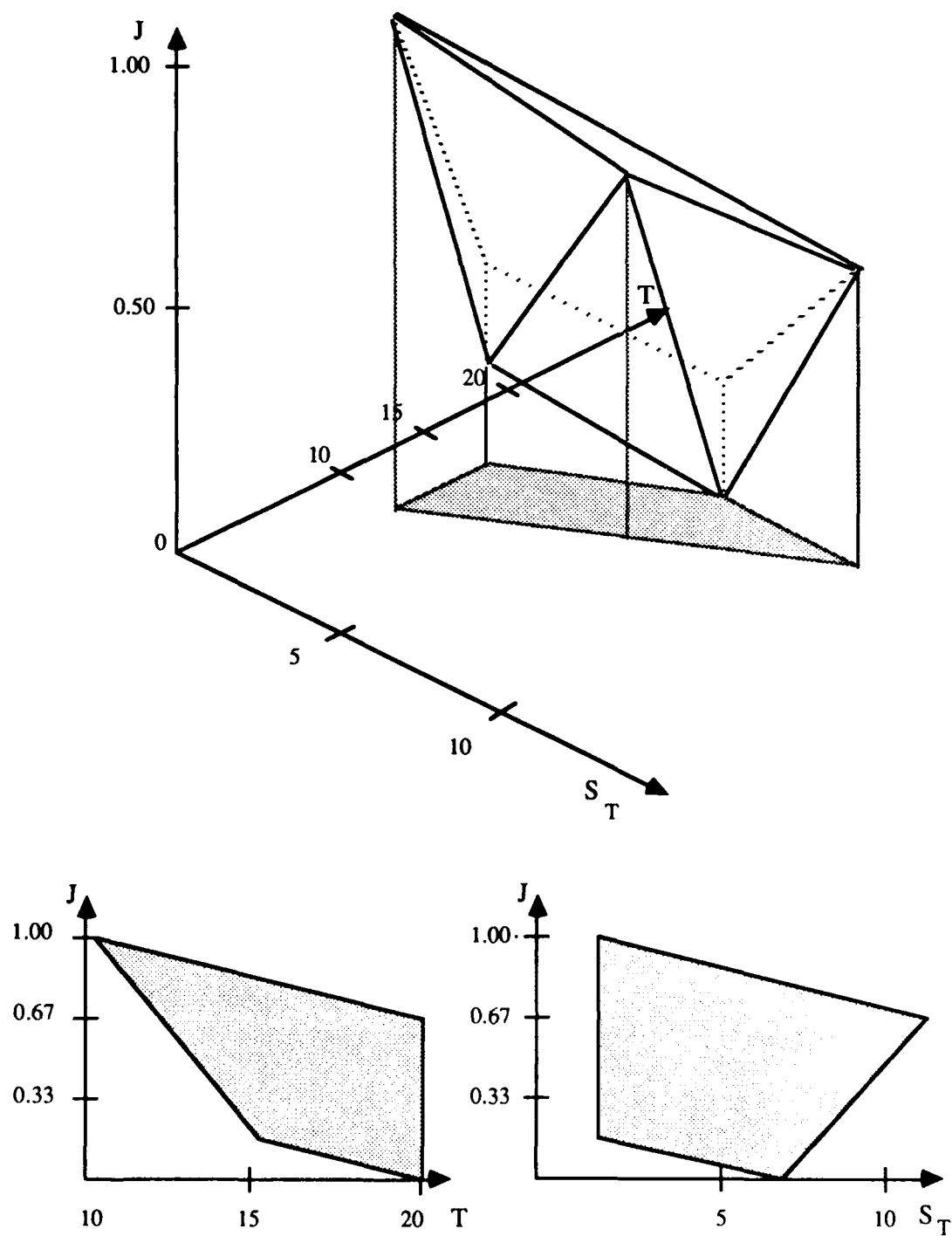
Fig. 7.5 Performance Locus in Case 2
