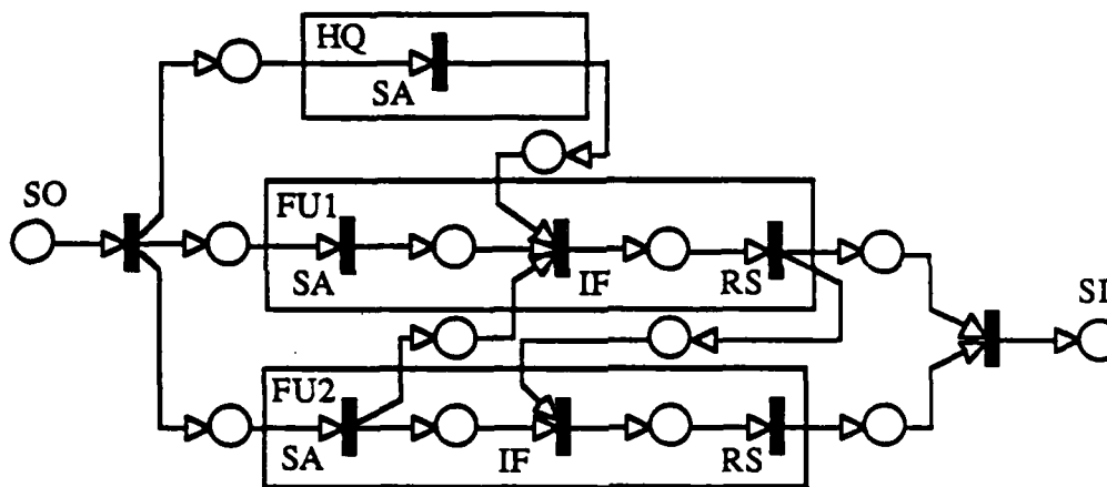
Figure 7.2 Candidate #2: FDMO2.
