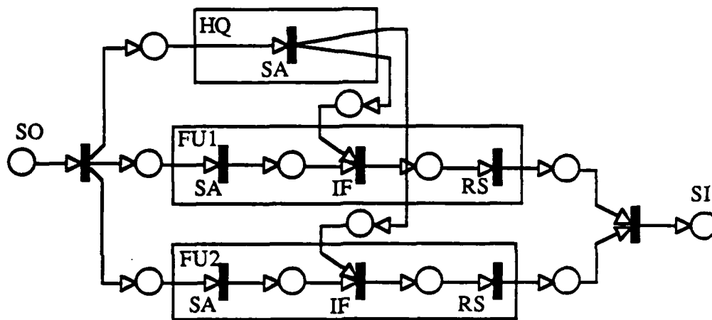
Figure 7.1 Candidate #1: FDMO1.
