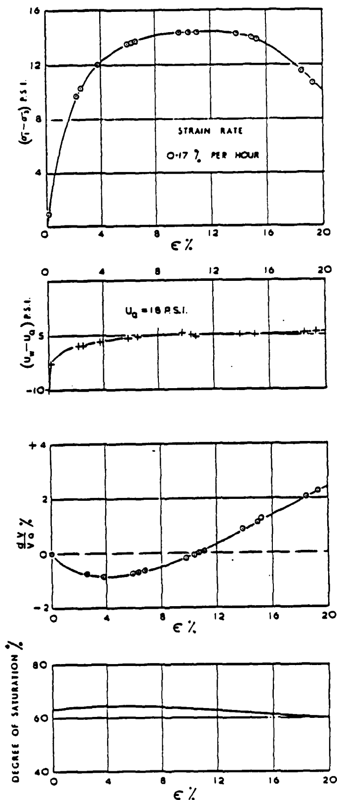
FIG. 2 CONSTANT WATER CONTENT TEST WITH CONTROLLED AIR PRESSURE ON PARTLY LOOSE SILT
