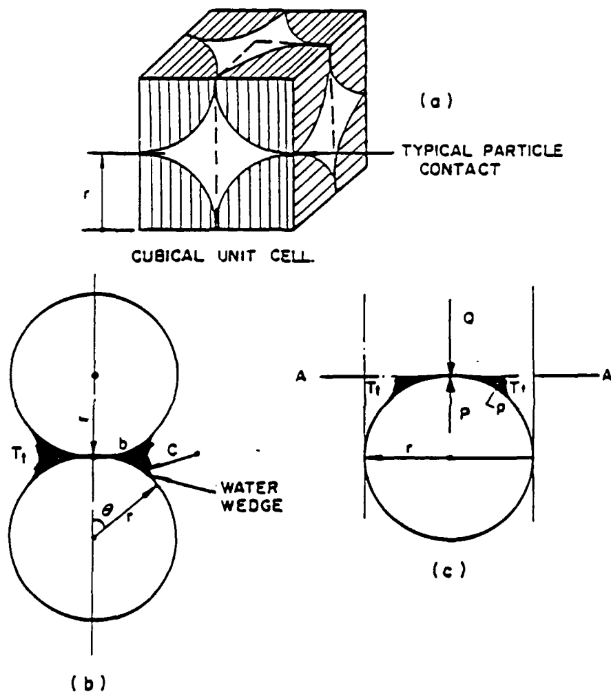
FIG. 1 TERMS USED IN ANALYSIS OF EFFECTIVE STRESSES IN IDEALIZED SOIL
