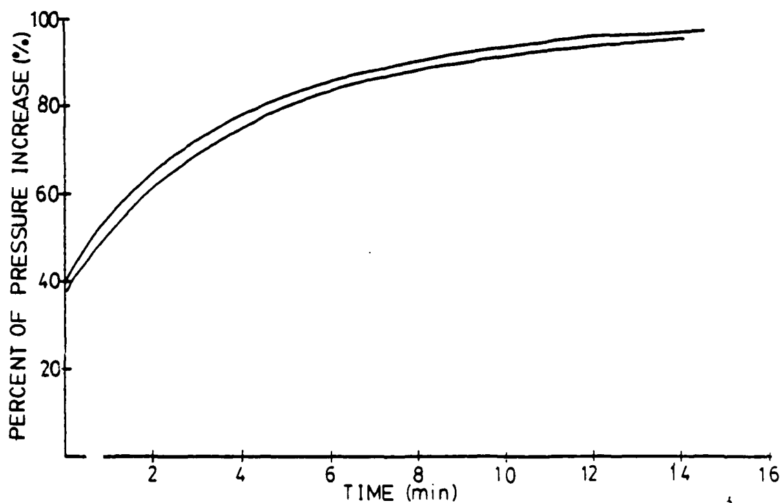
FIG.17 LAG TIME IN PRESSURE RESPONSE WITH CERAMIC STONE
