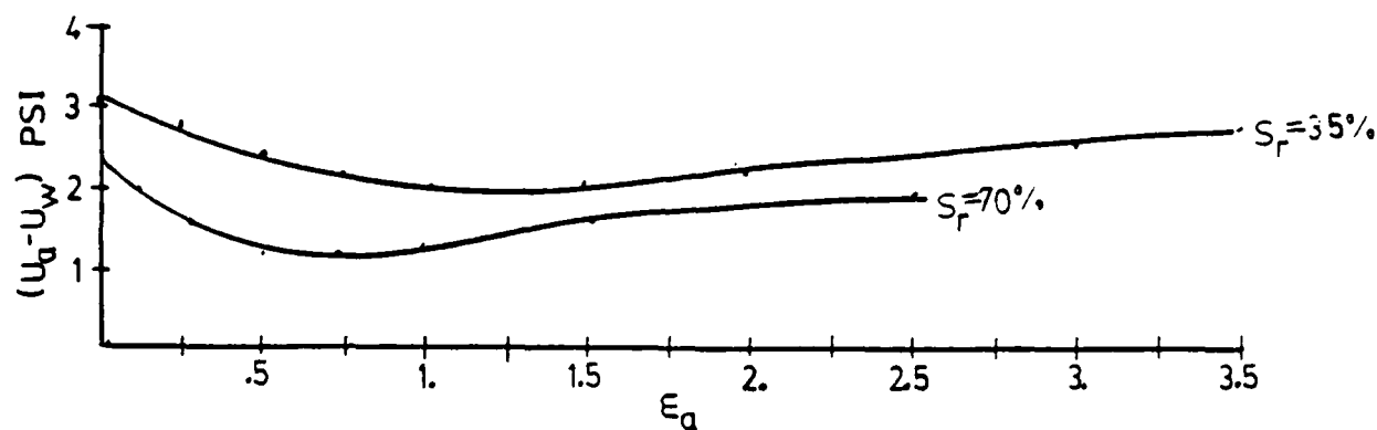
c) matrix suction vs. axial strain
