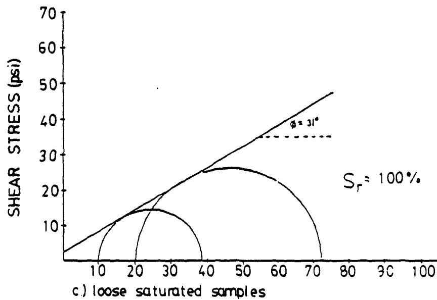
FIG.11 MOHR CIRCLE DIAGRAMS OF TEST RESULTS
