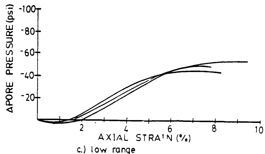
FIG.13 CHANGE IN PORE PRESSURES VS. AXIAL STRAIN FOR SATURATED SAMPLES
