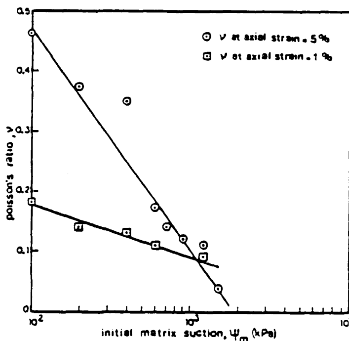
c) poisson's ratio as a function of initial matrix suction
