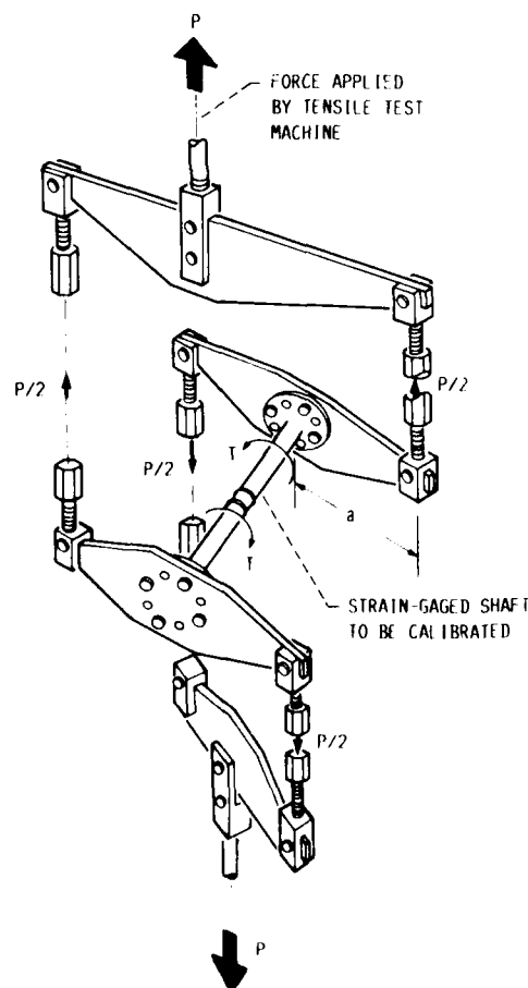
Figure 7.—Fixture used for shaft strain gage torque bridge calibration. Applied torque, T = Pa .
