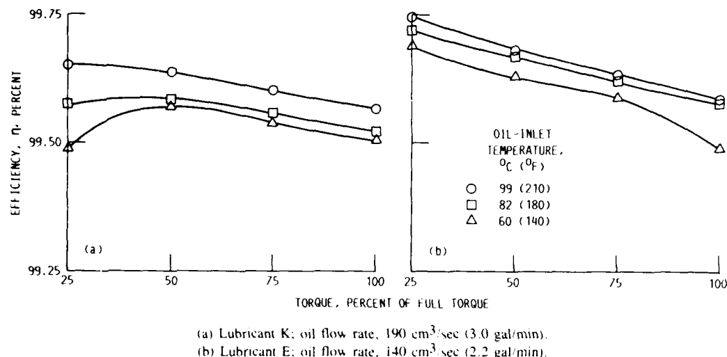
Figure 11.—Efficiency as function of torque at three oil-inlet temperatures. 100 percent speed, 1622 rpm.
