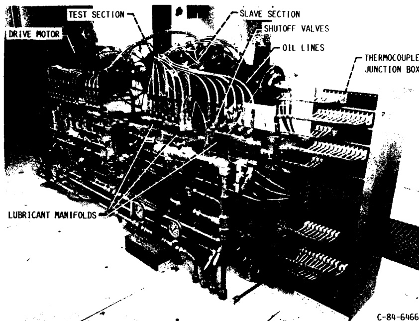
Figure 3.—Test facility showing lubrication distribution system.
