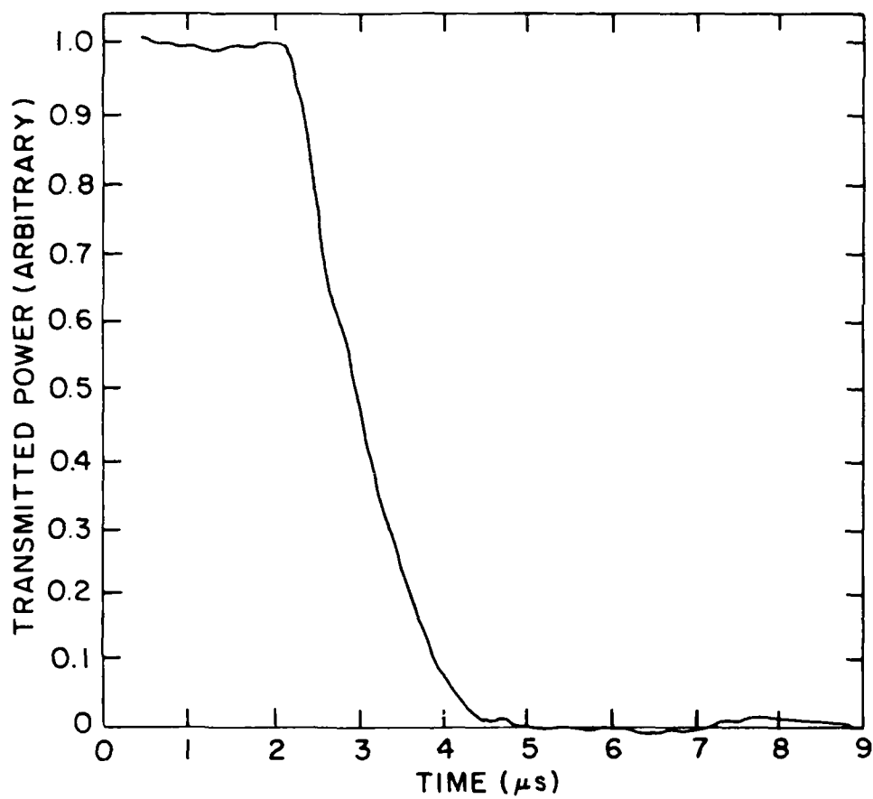
Fig. 9 Illustration of microwave transmission measurements at d=10 cm. The plasma density is > 6 \times 10^{13} \text{ cm}^{-3} at t \approx 2.5 \mu\text{s} (here, gun current starts at t = 2.0 \mu\text{s} ).
