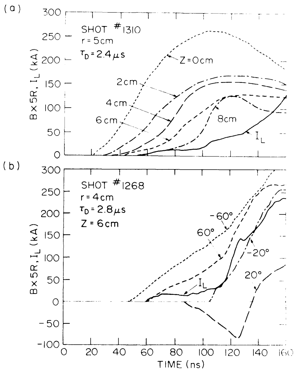
Fig. 24 (a,b) Same as Fig. 21(a,b), except for a slow opening angle.
