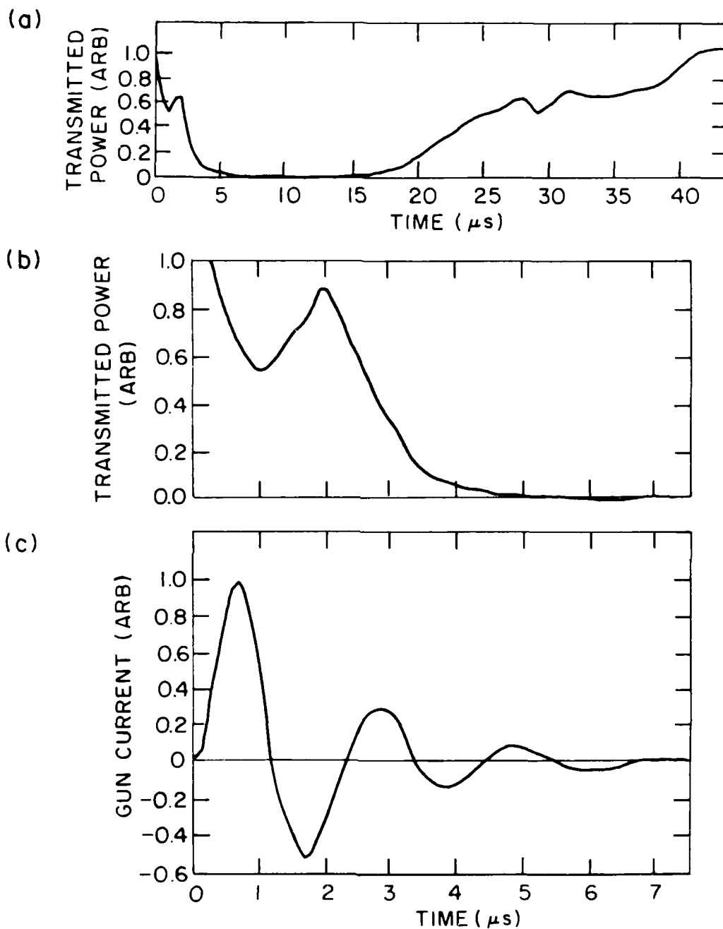
Fig. 8 Illustration of microwave cutoff measurements at d=20\text{cm} . The plasma density is > 6 \times 10^{13} \text{ cm}^{-3} at t \approx 5 \mu\text{s} .
