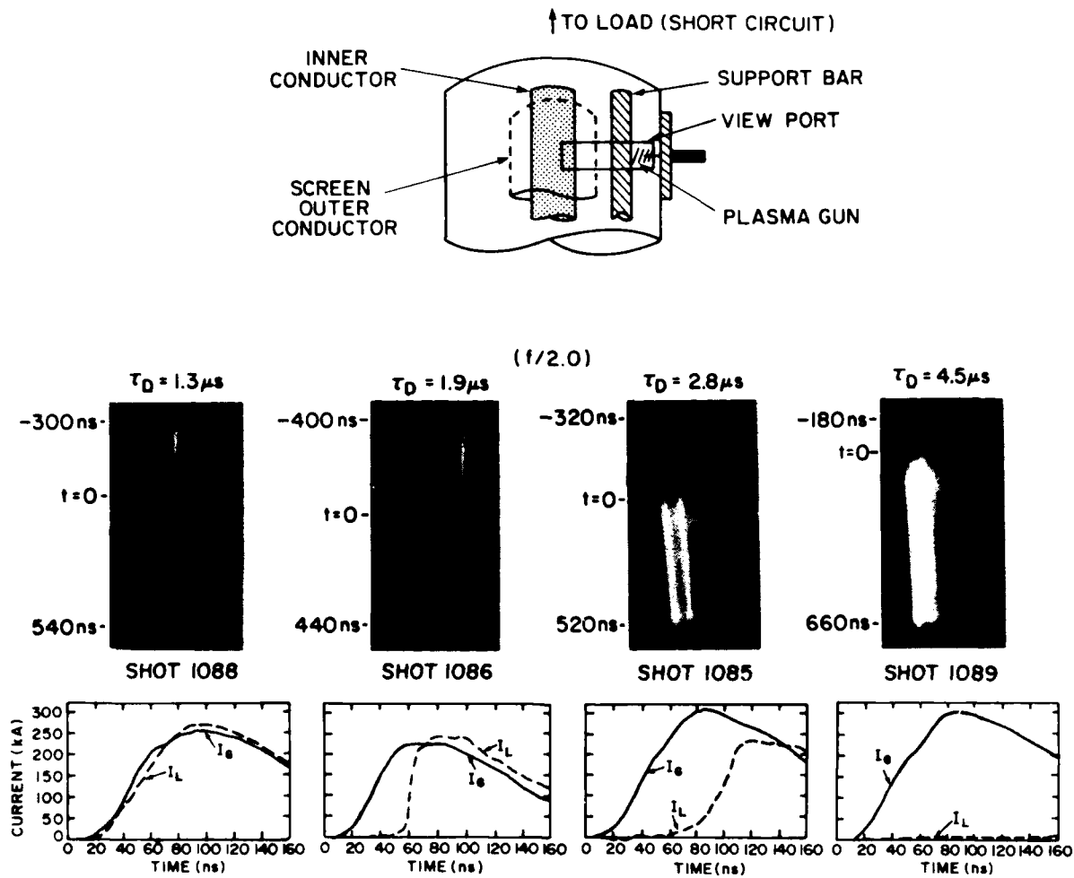
Fig. 14 Upper: Arrangement for streak camera photography during a shot on Gamble I. Middle, lower: Four streak photographs and current traces for various generator delay times.
