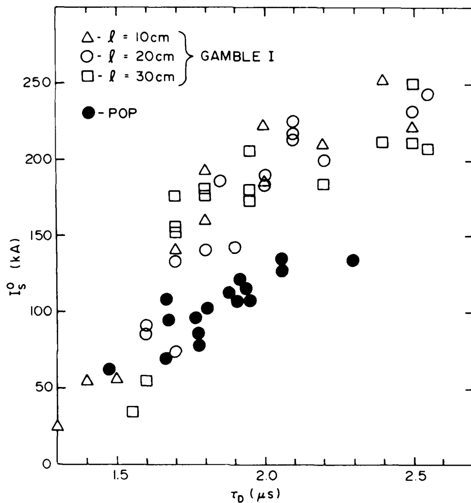
Fig. 21 Peak switch current, I_s^0 , as a function of relative delay time, \tau_D , for 10-20-, and 30-cm long switch where n_{i1} was constant for each \tau_D . Also shown are results with the same n_{i1} but a factor 10 longer conduction time (POP).
