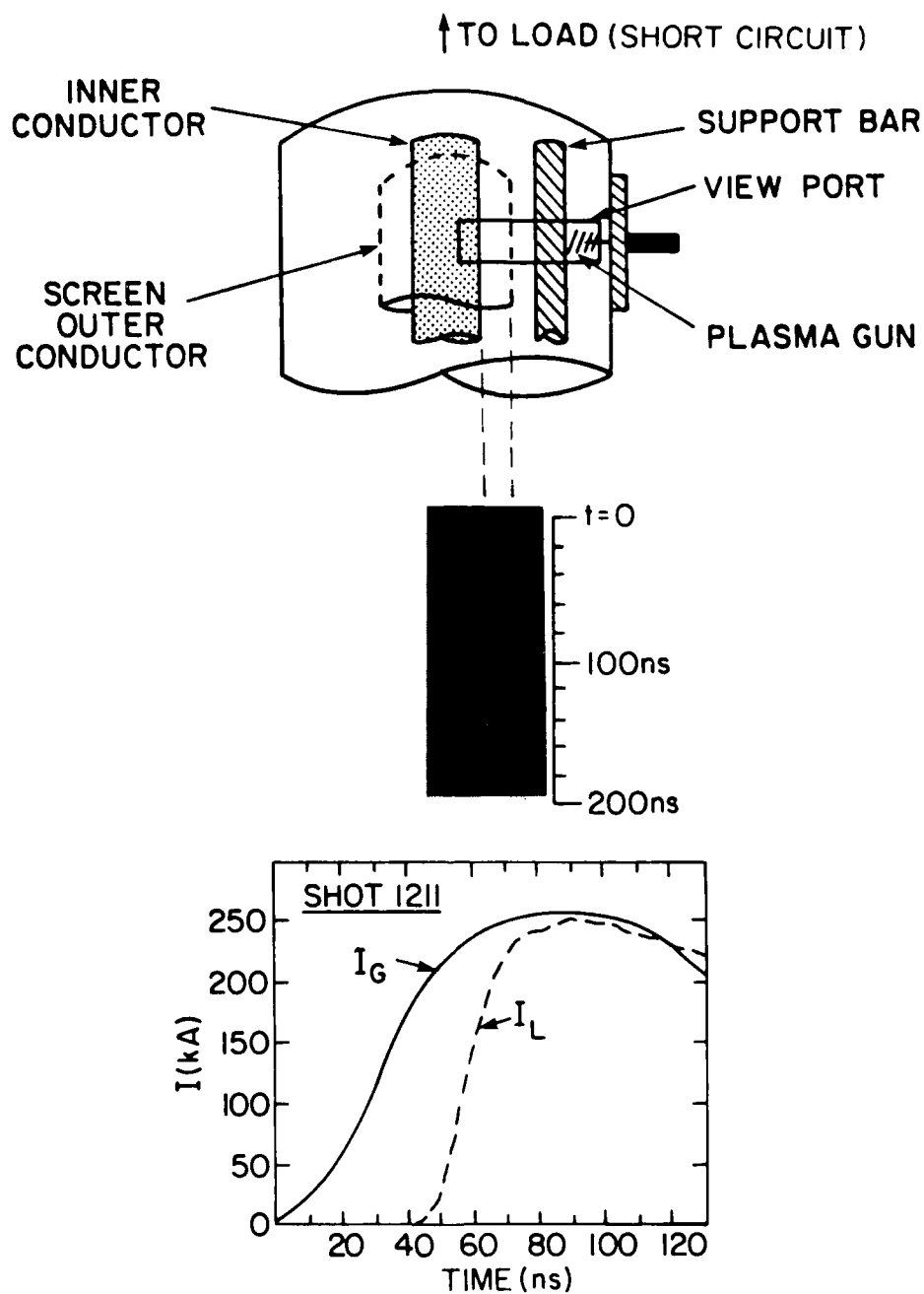
Fig. 15 Upper: Arrangement for fast streak camera photography during a shot on Gamble II. Middle, lower: Fast streak photograph and current trace.
