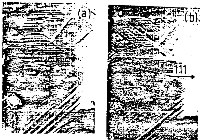
Fig.6: Optical micrographs of domain structure on (112) surface in zero field at a) 260K and b) 315K.
