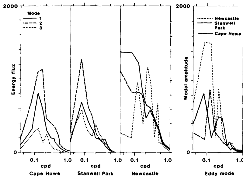
FIG. 8. Spectra of the amplitude of the first three CTW modes at Cape Howe, Stanwell Park and Newcastle. These spectra are normalized such that the area under the curve is proportional to 2f/\rho_0 times the energy flux. The spectra of the eddy mode at Cape Howe, Stanwell Park and Newcastle are also shown. Note that the currents were not high-passed filtered before obtaining these spectra.
