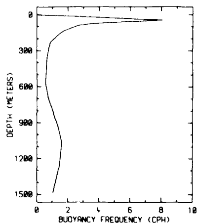
Fig. 2. Mean buoyancy frequency profile. The profile is a smoothed representation of a profile calculated by Pennington and Briscoe [1979] from conductivity, temperature, and depth casts during the experiment.
