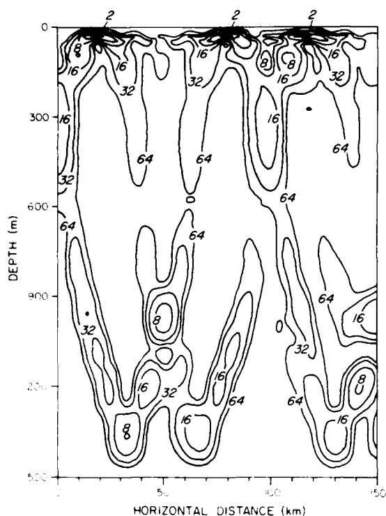
Fig. 16 Minimum Richardson number ( N^2 / (g' / (Cz)^2) ) over a tidal cycle calculated from the velocity field.
