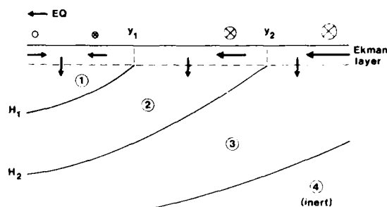
FIG. 1. A schematic meridional cross section of the layer structure of the model. The base of the n th layer outcrops at y_n .
