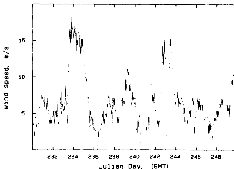
Fig. 5. Wind speeds measured from R/V Oceanographer during the MILE experiment. There are two major storms evident in the wind record, the strongest on days 234–235, the other on day 243.
