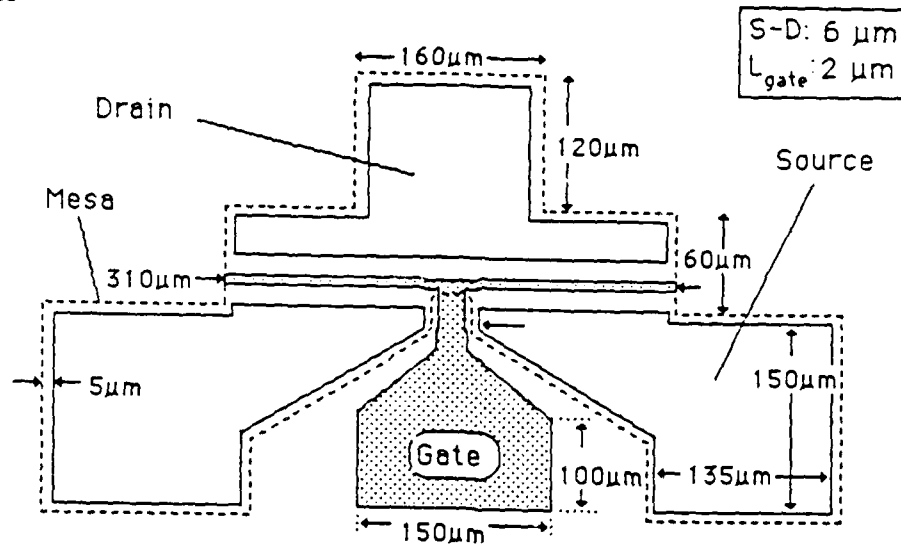
a) Schematic of the UCSD 2 \mu\text{m} gate FET
