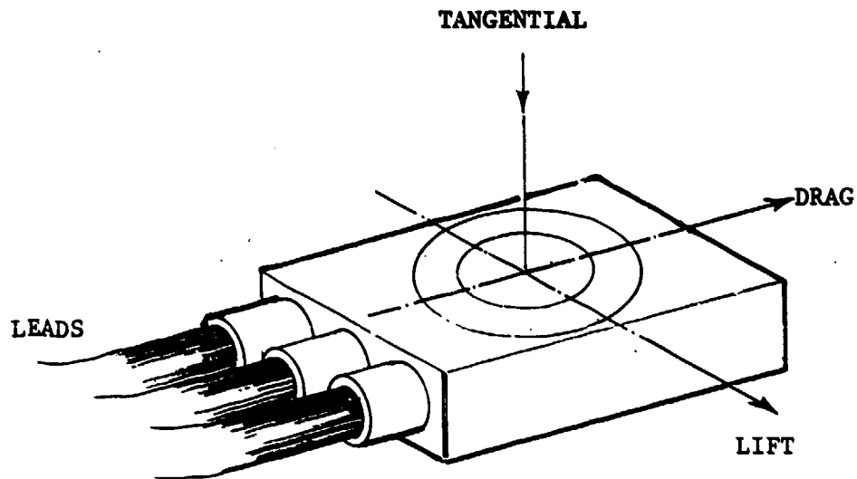
FIGURE 14. QUARTZ FORCE TRANSDUCER
