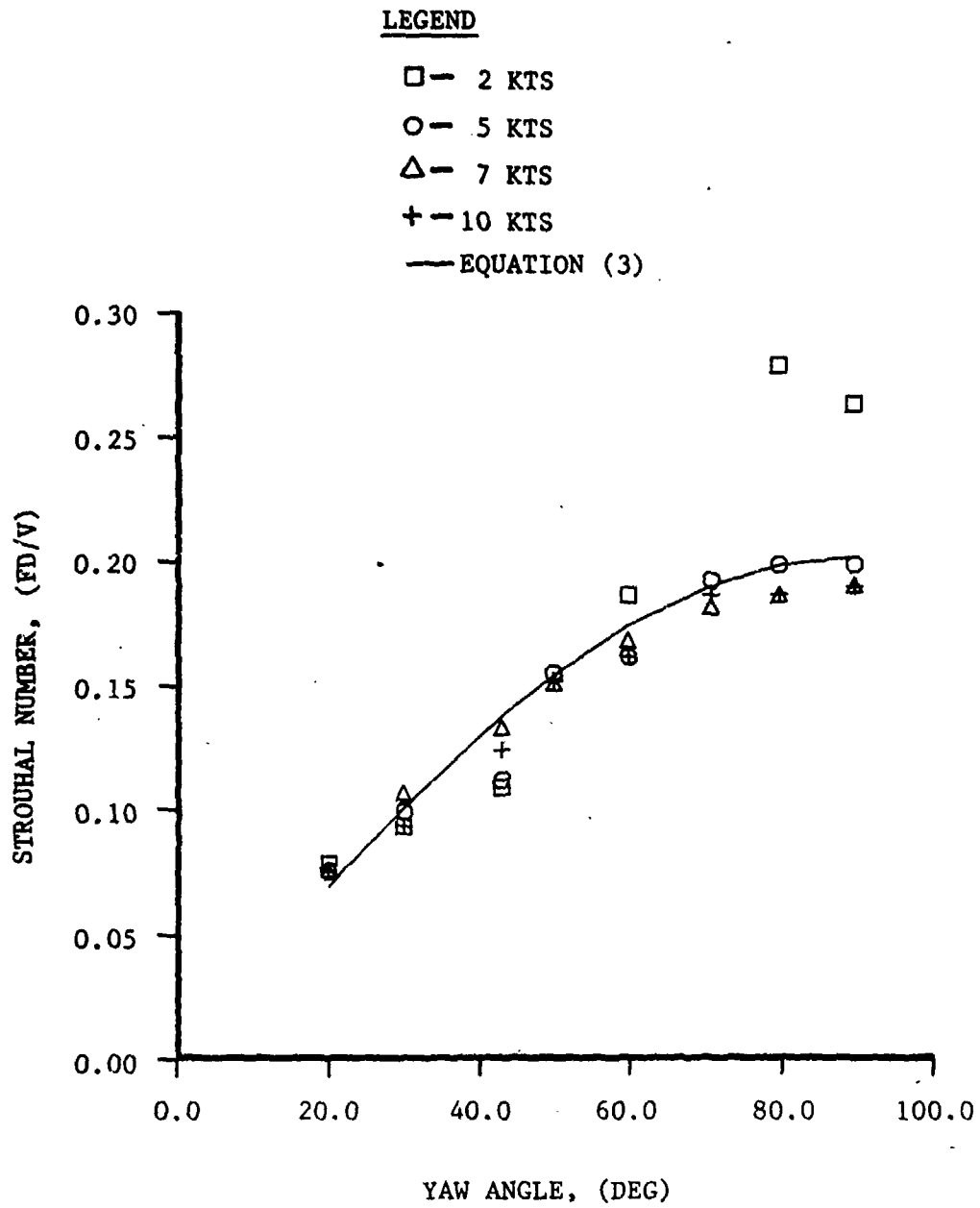
FIGURE 40(a). COMPARISON OF MEASURED CABLE STROUHAL NUMBERS AND PREDICTED STROUHAL NUMBERS VERSUS YAW ANGLE AT HIGH TENSION 1 x 19 CABLE (Sheet 1 of 4)
