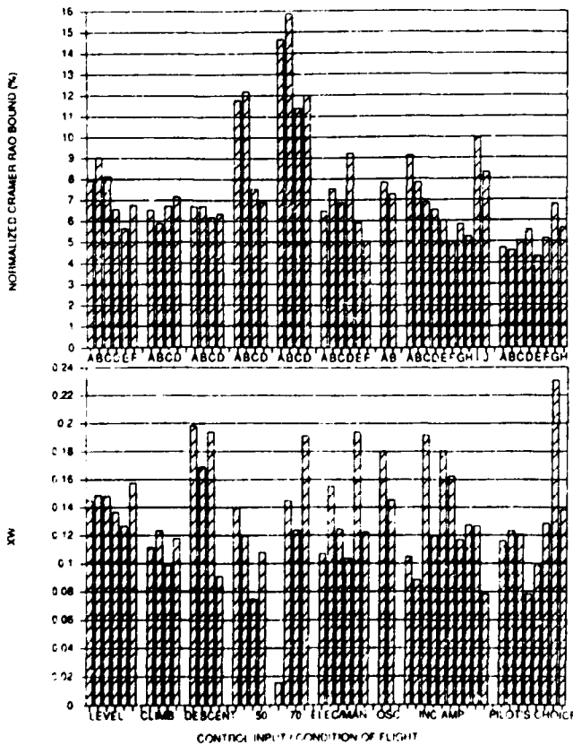
Stability Derivative - X_w
