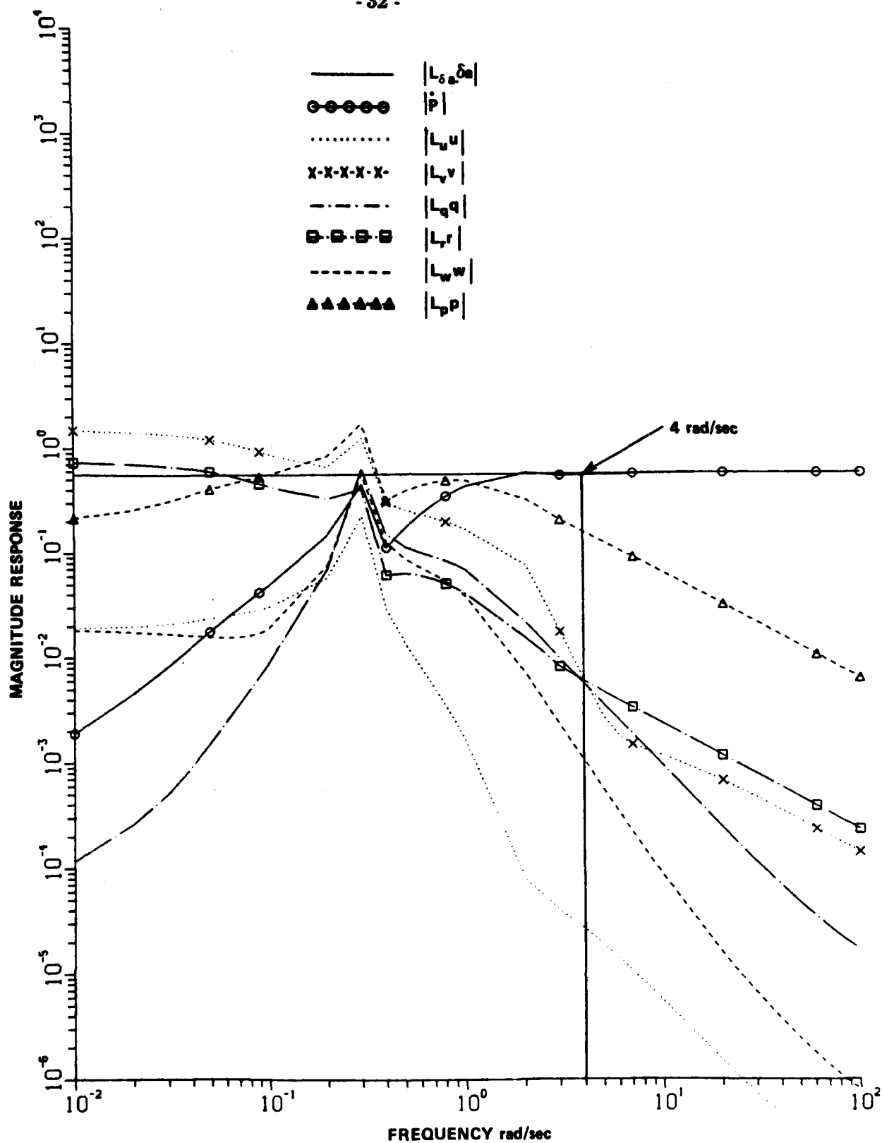
FIG. 7: BODE PLOT - ROLL RESPONSE
