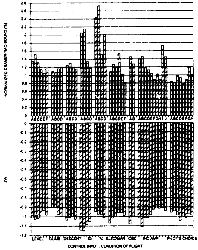
Stability Derivative - Z_w
