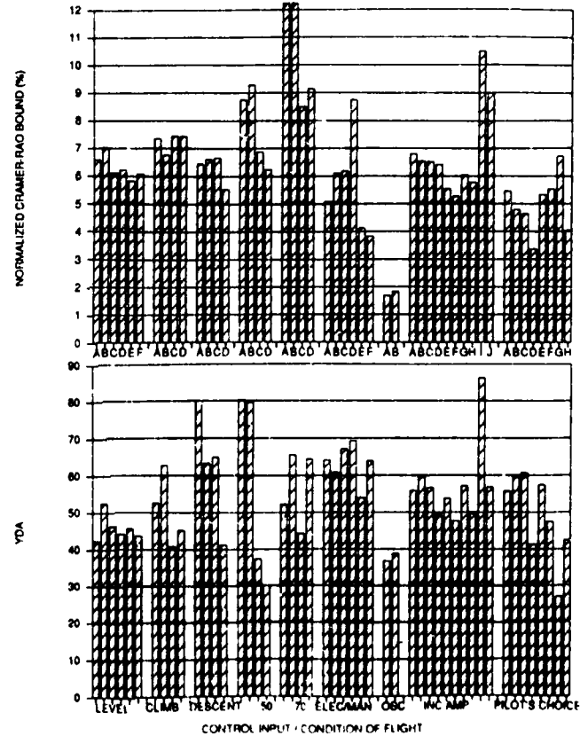
Control Derivative - Y_{da}
