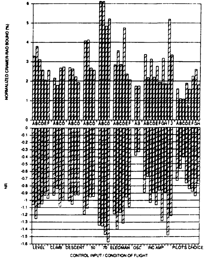
Control Derivative - N_{\dot{r}}
