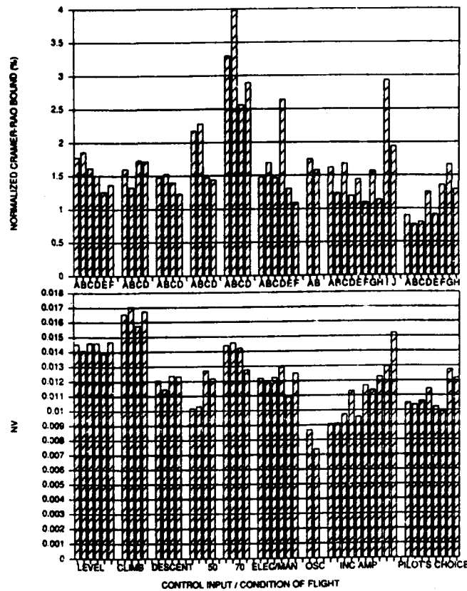
Control Derivative - N_{\dot{\alpha}}
