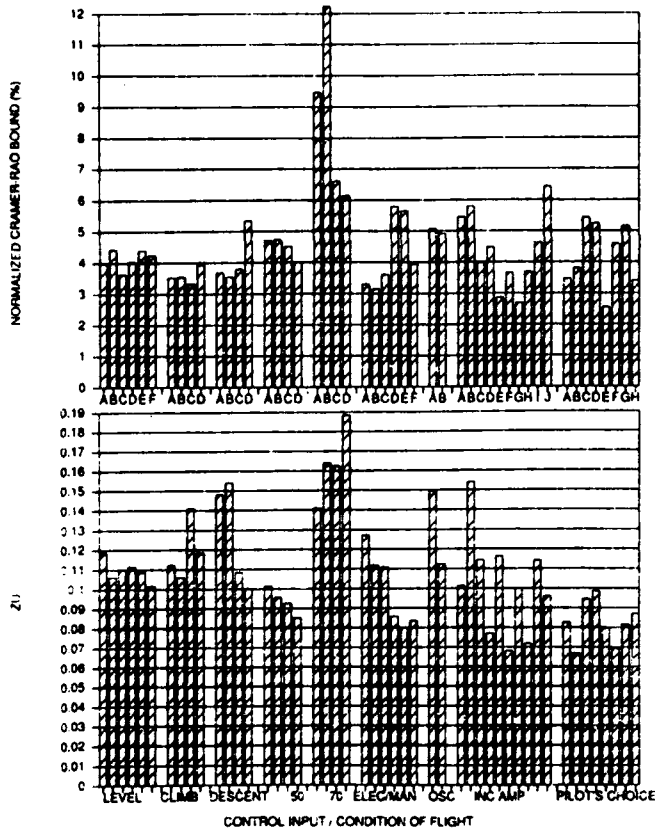
Stability Derivative - Z_u
