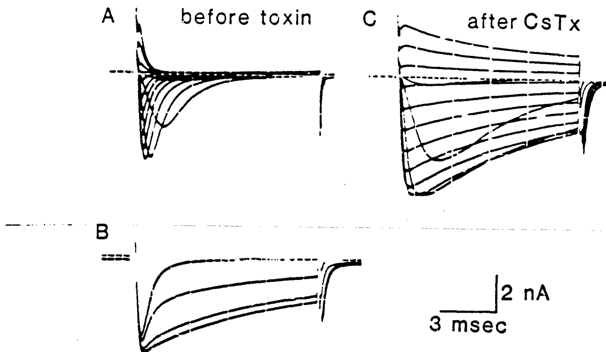
Figure 6. Effect of CsTx on the time course of sodium currents. A. A high resistance seal was formed on an N18 cell. After 20 min at a holding potential of -80 mV, the cell was hyperpolarized to -120 mV for 100 msec and depolarized for 10 msec to test potentials of -50 mV to +80 mV, in intervals of 10 mV, once per second to elicit the sodium currents illustrated. B. Eighteen \mu l of 4 \times 10^{-6} M CsTx were added to the recording medium approximately 7 mm from the cell to give a final concentration in the recording bath of 1 \times 10^{-7} M. Sodium currents were elicited every 30 sec by hyperpolarizing to -120 mV for 100 msec and depolarizing to +10 mV for 10 msec. Superimposed traces from a storage oscilloscope are shown. C. Six min after addition of CsTx, a family of sodium currents was recorded as in panel A.
