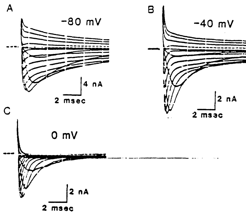
Figure 9. Voltage-dependence of CsTx action between -80 and 0 mV. A. N18 cells were incubated in the presence of 3 \times 10^{-8} M CsTx at 37° C for 30 min. An individual cell at a holding potential of -80 mV was hyperpolarized to -120 mV for 200 msec and a family of sodium currents was elicited by 10 msec test pulses to potentials of -50 to +80 mV in intervals of 10 mV. B. The holding potential was changed to -40 mV for 5 min and a family of sodium currents was recorded as in A. C. The holding potential was then changed to 0 mV for 5 min and a family of sodium currents was recorded as in A.
