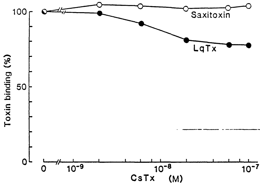
Figure 13. Effect of CsTx on binding of saxitoxin and Leirus scorpion toxin to sodium channels. Specific binding of [ ^3\text{H} ]saxitoxin (○) and [ ^{125}\text{I} ]LqTx (●) to sodium channels in rat brain synaptosomes was measured in the presence of the indicated concentrations of CsTx.
