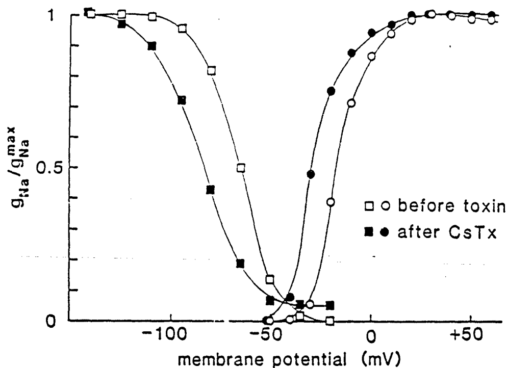
Figure 8. Effect of CsTx on the voltage-dependence of sodium channel activation and inactivation. Activation. Families of sodium currents were recorded in the presence and absence of 1 \times 10^{-7} M CsTx as described in the legend to Fig. 6. Peak conductance values were calculated and plotted as the ratio of the measured value to g_{Na} observed in a pulse to +30 mV (before toxin, \square ; after toxin, \bullet ). Inactivation. N18 cells were hyperpolarized for 100 msec to the indicated membrane potentials and then sodium currents were elicited by a test pulse to +10 mV for 10 msec. Conductance values were calculated and plotted relative to the sodium conductance observed after a prepulse to -140 mV (before toxin, \square ; after toxin, \blacksquare ).
