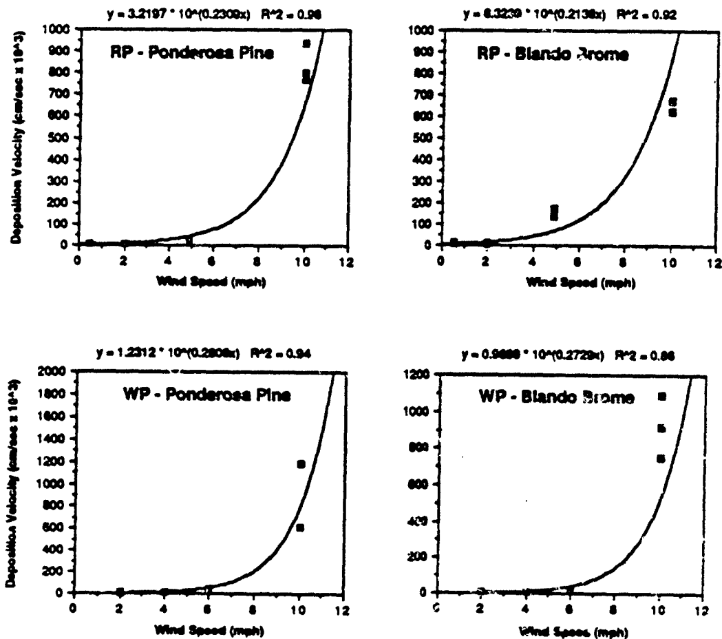
FIGURE 3.22. RELATIONSHIP BETWEEN WIND SPEED AND DEPOSITION VELOCITIES FOR PONDEROSA PINE AND BLANDO BROME FOLIAGE EXPOSED TO RP/BR AND WP SMOKES. SEE TABLES 3.37 AND 3.38 FOR PARTICLE SIZE DATA.
