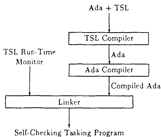
Figure 1: TSL Front-End.
