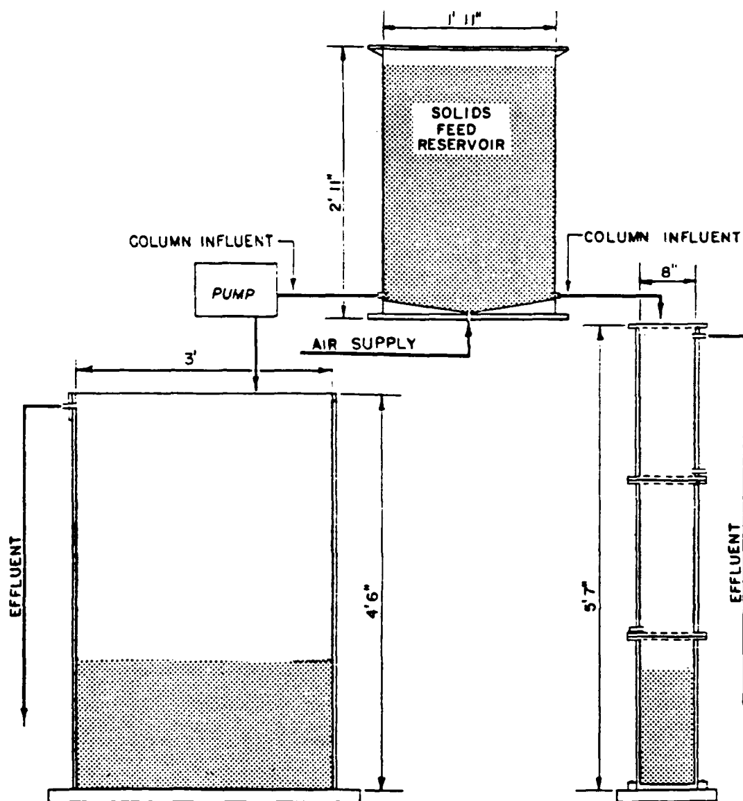
Figure 22. Column sedimentation test equipment used for Mobile Harbor sediment (Montgomery 1979)
