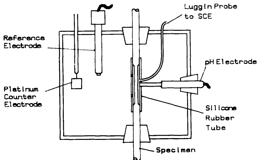
Figure 1. Configuration of CERT Test with Occluded Cell.
