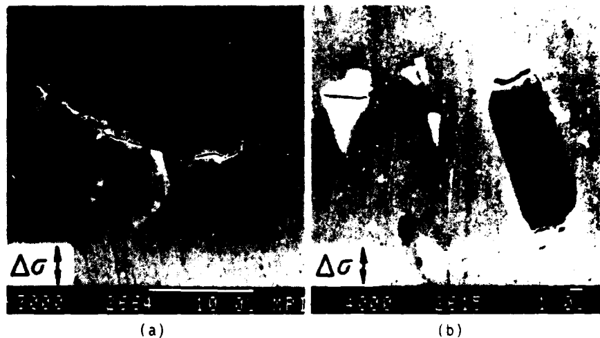
Fig. 15. SEM micrograph from the surface of fatigued AlMgSi1 samples (coarse dispersoid distribution). a) Cracks initiated in the transverse interfaces of two inclusions. b) Overloaded specimen showing a cracked inclusion and another one with decohesion of the transverse interface.
