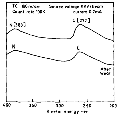
Figure 4 AES profiles illustrating N + migration
