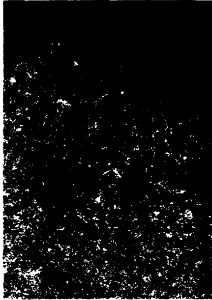
Figure 3 Crack deflection at MnS stringers (x 150)
