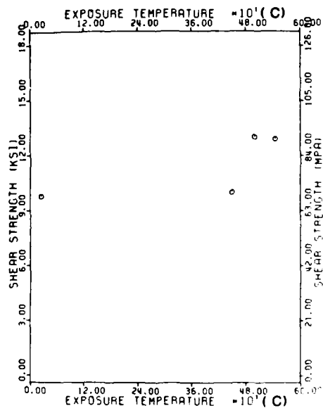
Figure 11 The effect of heat treatment on interfacial shear strength of Gr/201 Al composite
