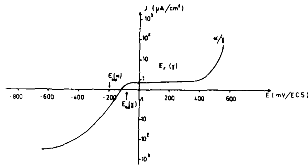
Figure 1 Polarization curve of the \alpha/\gamma duplex alloy in the 3.5 % NaCl solution at pH 2 and \Delta E/\Delta t = 90 mV/h.
