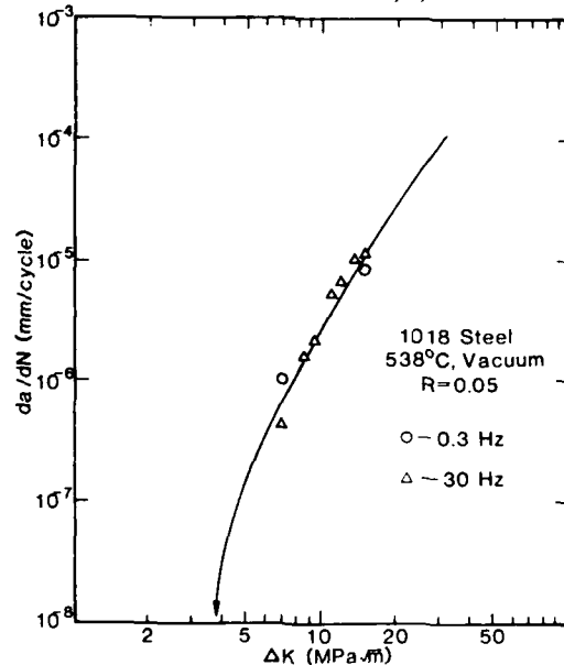
Fig. 8b da/dN data for 1018 steel as a function of frequency compared with behavior of ferritic steels shown in Fig. 8a, solid line.
