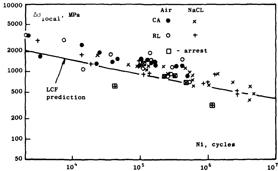
Figure 2 Prediction of Initiation Life from LCF Properties for 817M40 Steel
