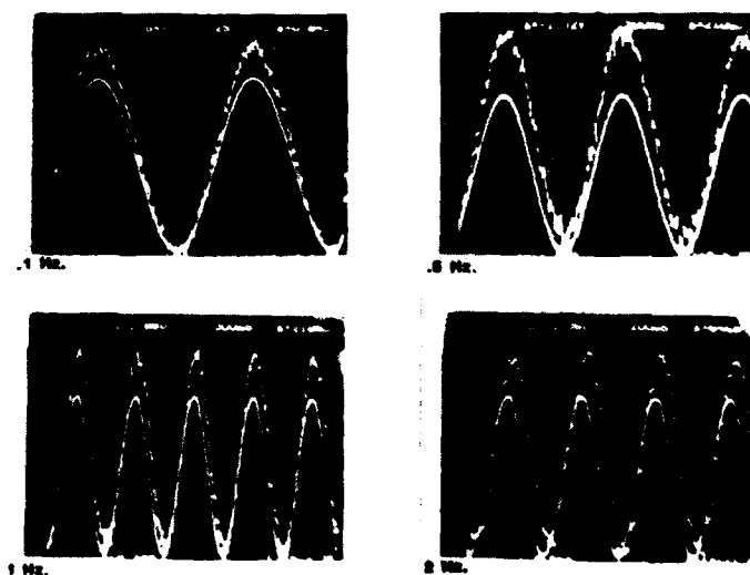
Figure 2 Oscilloscope traces of strain vs. time from the laser system compared with load vs. time
