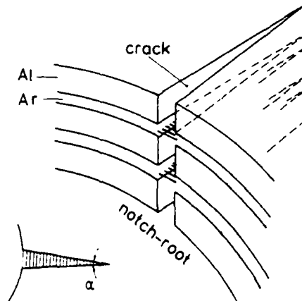
Figure 2 Crack bridging in ARALL (schematic)
