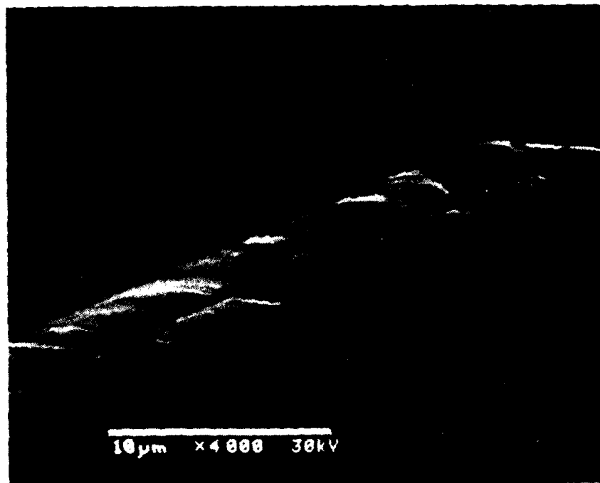
Figure 3. SEM observation of microcracks and intrusions
