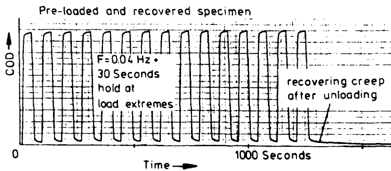
Figure 7 Time dependent behaviour of the COD due to adhesive shear deformation
