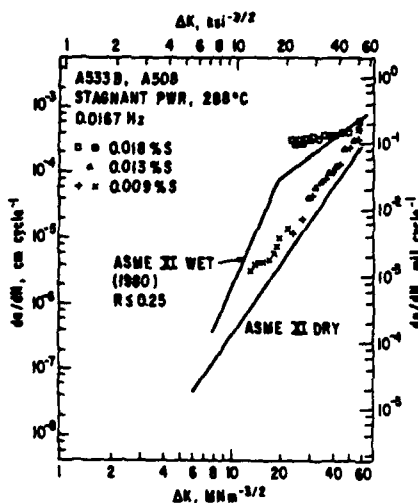
Figure 1. Effect of S content on da/dN vs \Delta K , R=0.2 , triangle (11).
