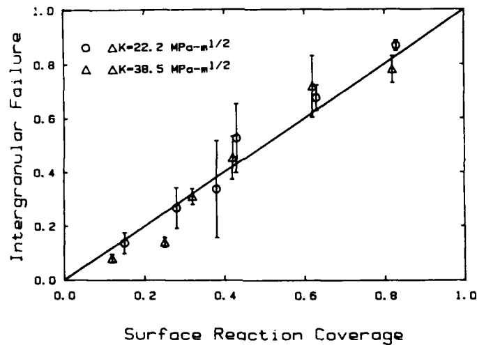
Figure 9 Correlation between surface coverage and fraction of intergranular failure (or \phi ) for AISI 4340 steel.
