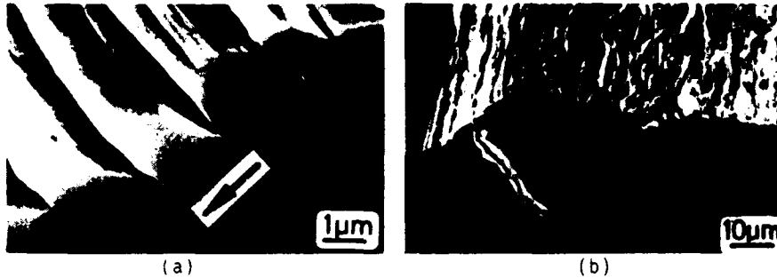
Fig. 12. SEM micrographs of longitudinal sections of fatigued Cu single crystals (undistorted view) and part of the surface (20 Hz, \gamma_{01} = 0.2\% ). Courtesy of Hunsche and Neumann (62)
