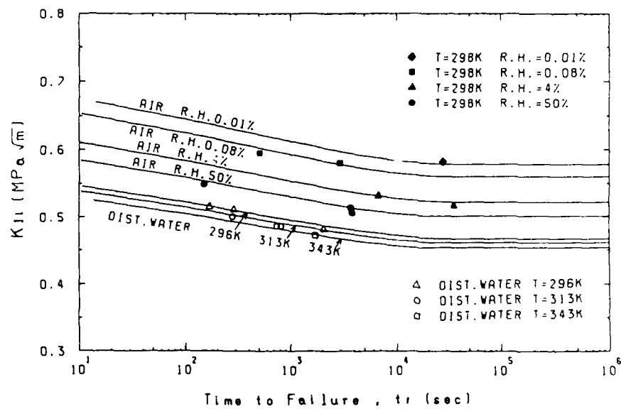
Figure 7 Initial stress intensity factor, K_{Ii} , vs. time to failure, t_f
