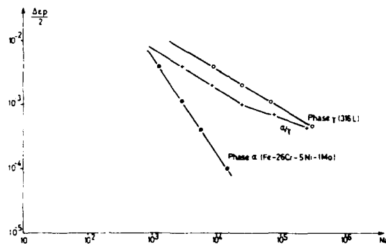
Figure 2 Coffin-Manson curves, in air at \dot{\epsilon} = 10^{-2} s^{-1} of the \alpha/\gamma duplex alloy and of its \alpha and \gamma phases considered separately.
