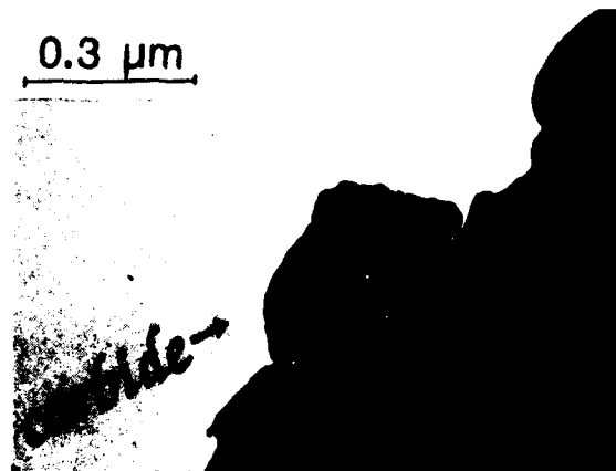
Figure 3 Micrograph revealing the presence of an \text{Al}_4\text{C}_3 particle for specimen heat treated at 545^\circ\text{C}
