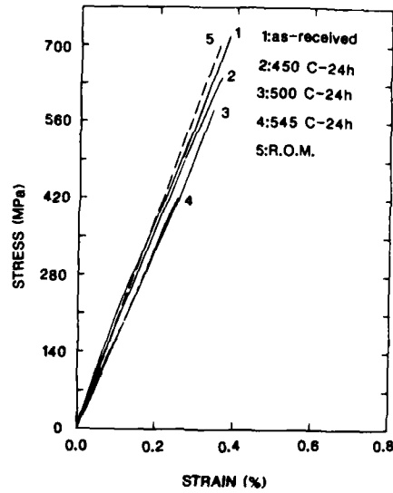
Figure 4 Representative tensile stress-strain curves obtained for Gr/201 Al composite specimens
