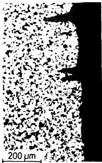
Fig.7 Oxide wedge on the outer side of the pipe of a steam superheater
