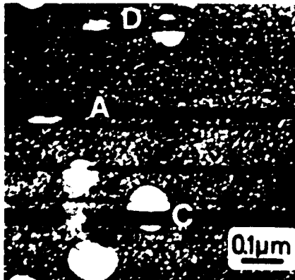
Fig. 10. Dark field TEM micrograph of an fatigued Nimonic 80A alloy. Dark bands are no PSBs but tilted areas between two active slip planes with opposite cumulative shear (55).
