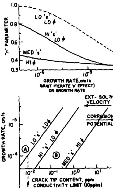
Figure 5. Predicted effect of metall. S on crack tip chemistry.
