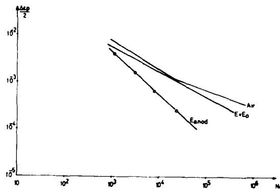
Figure 3 Coffin-Manson curves at \dot{\epsilon} = 10^{-2} s^{-1} of the duplex alloy at E = E_0 and E = +150 mV (ECS \equiv saturated calomel electrode)
