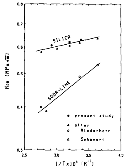
Figure 6 Environmental fracture toughness, K_{Ic}
