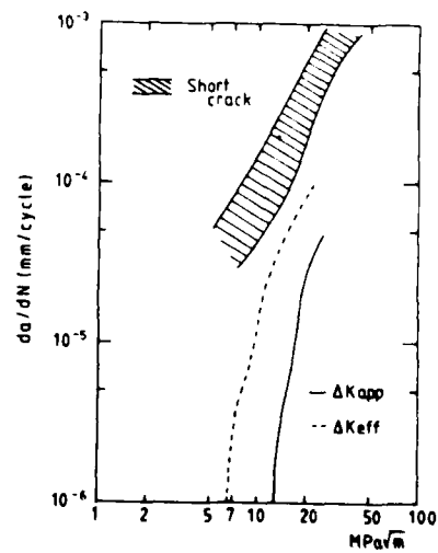
Figure 17 Small and long fatigue crack growth for the titanium alloy IMI 685.
