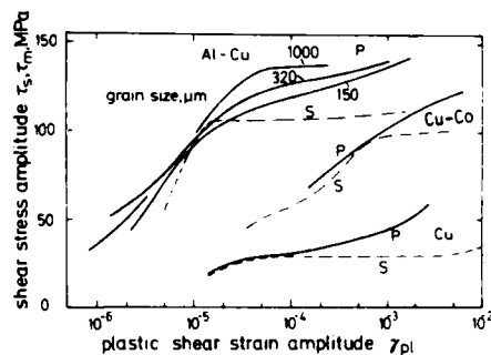
Fig. 11. Comparison of cyclic stress-strain curves from single and polycrystals of Al-Cu containing \theta'' (58) under-aged Cu-Co (60) and pure Cu (26). For stress and strain correction the Sachs factor 2.24 has been used.
