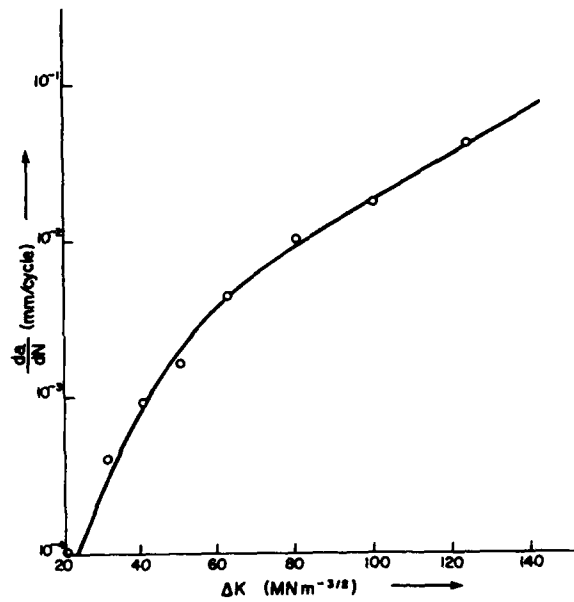
Figure 2. Fatigue of a Ti-alloy in seawater.
