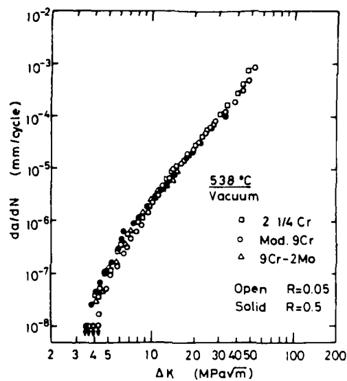
Fig. 8a da/dN vs. \Delta K plot for three ferritic steels in vacuum at 538°C as a function of R (%).
