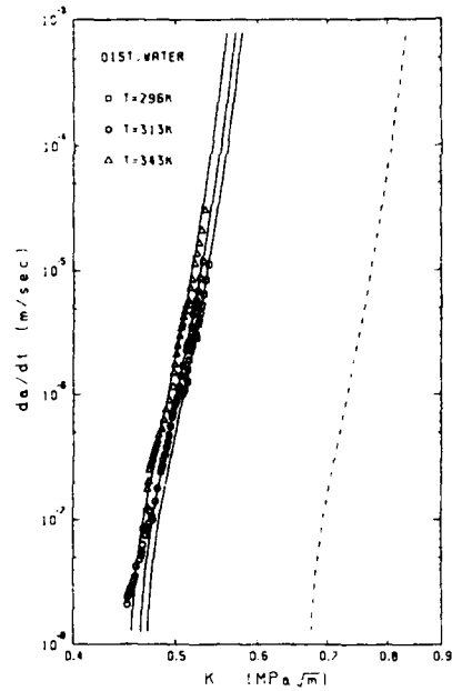
Figure 5 da/dt -K in a distilled water
