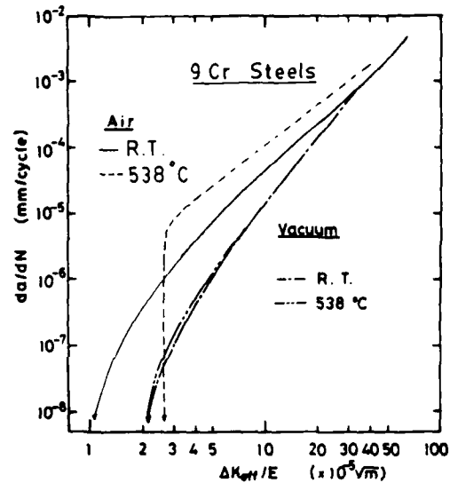
Fig. 9 da/dN as a function of \Delta K/E for a modified 9Cr-1Mo steel tested in air and in vacuum at room temperature and 538°C (9).
