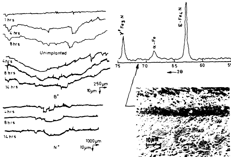
Figure 5 Typical wear track profiles
