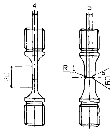
Fig.1 Notched specimen geometry.
