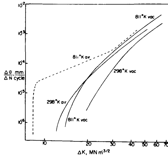
Fig. 6 da/dN vs. \Delta K plots for Ti-6Al-2Sn-4Zr-2Mo-0.1Si alloy at R=0.05 at room and elevated temperatures in air and in vacuum (7).
