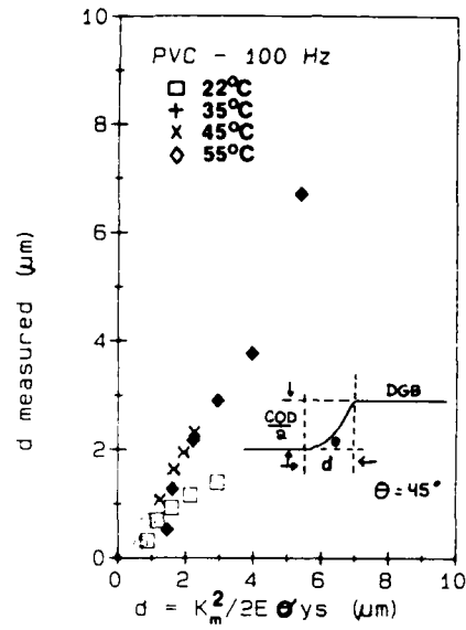
Figure 5. Correspondence of Measured and Calculated Stretch Zone Width Values.
