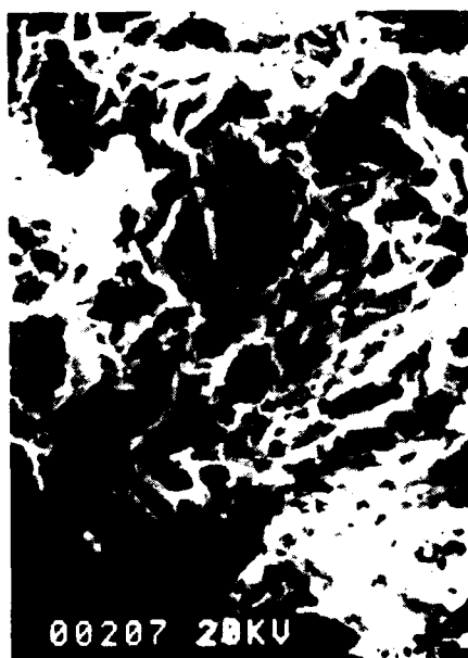
Figure 5. Fracture Surface Observed at -1200 mV (SCE).
