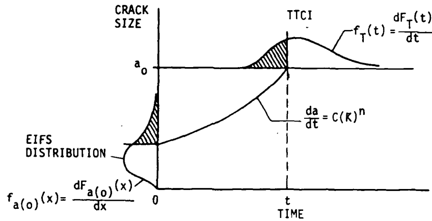
Figure 10 Relation between TPCI and EIFS
