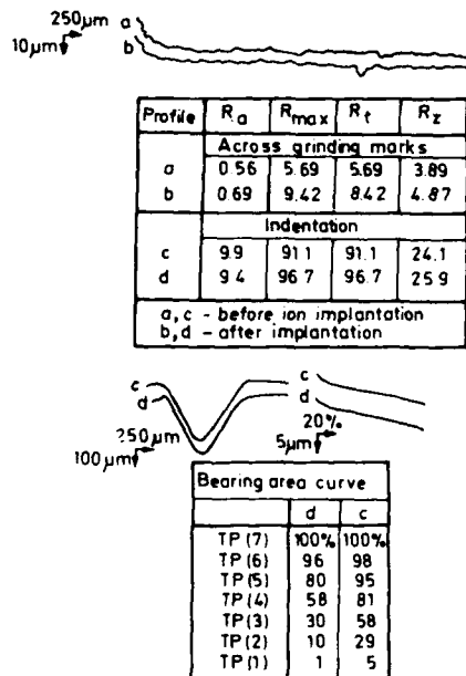
Figure 1 Bearing area improvement & valley deepening on implantation
