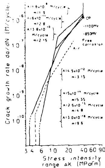
Figure 10. Mean crack growth curves for different conditions R=0.5 (7).
