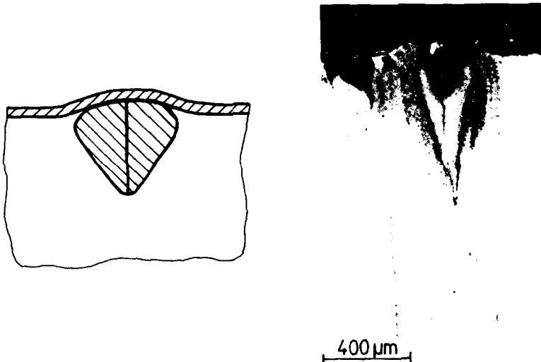
Fig.3 Oxide wedge under the unaffected layer of the metal/oxide composite Fig.4 Metal deformation alongside the oxide wedge. A crack through the surface composite and the wedge
