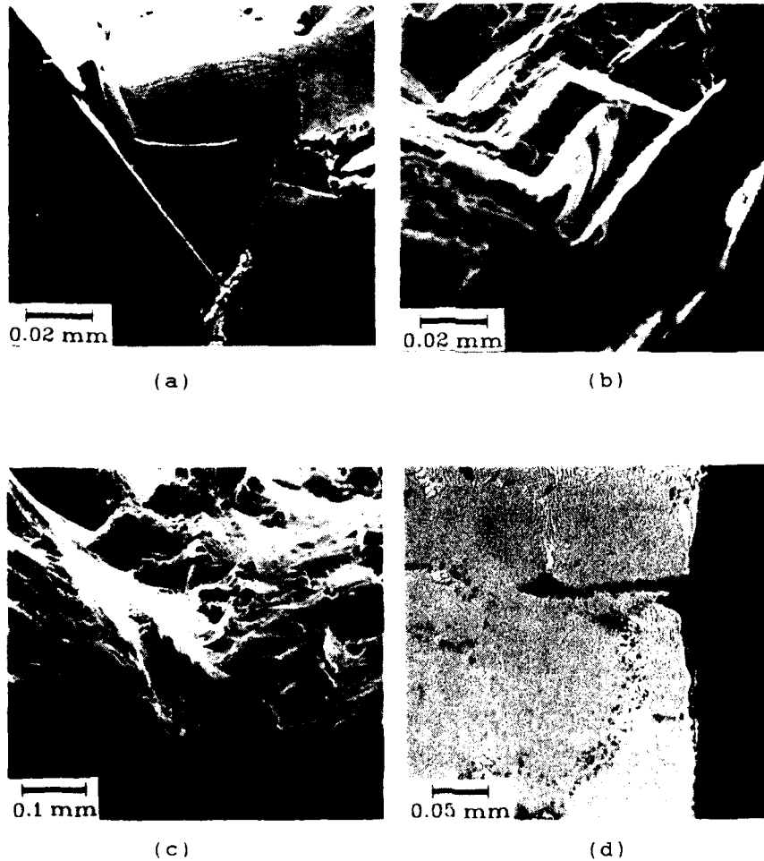
Figure 12. LCF fracture behavior of MAR-M 246. (a) Initiation and crystallographic propagation at 20°C. (b) Less crystallographic fracture at 704°C, 100%/min. (c) Initiation due to oxidation at 927°C. (d) 927°C oxide spikes.
