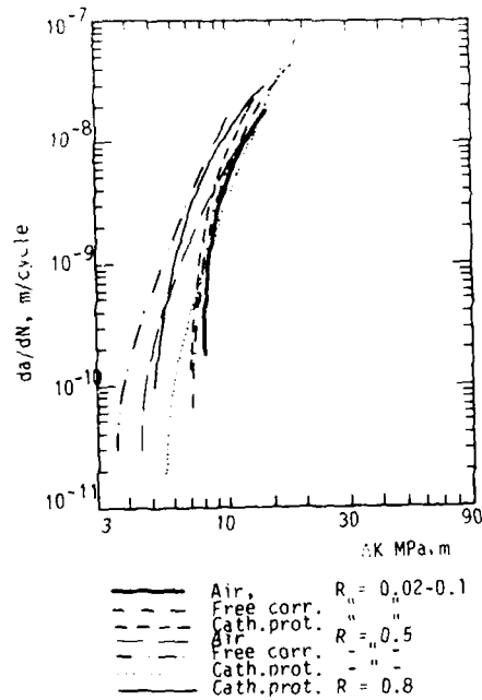
Figure 2. Mean crack growth curves for different experimental conditions.
