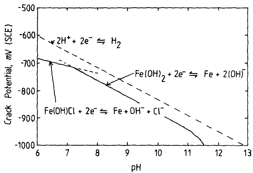
Figure 7. Schematic E-pH Behaviour in a Crack.
