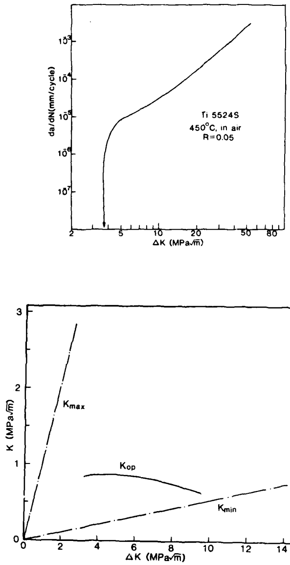
Fig. 7 da/dN and crack opening behavior for Ti 5Al-5Sn-2Zr-4Mo-0.25Si in air at elevated temperature (8).
