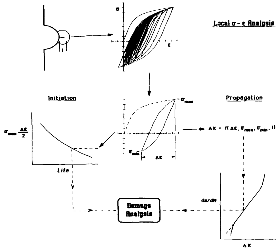
Figure 9 Details of local stress-strain and damage analysis
