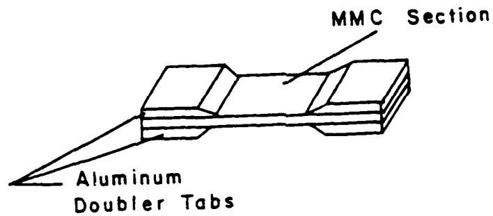
Figure 1 Composite specimen configuration
