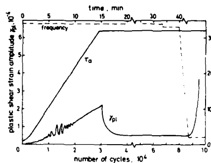
Fig. 2. Shear stress and plastic shear strain response of a copper single crystal. Ramp loading at 34 Hz to a constant stress level. Final reduction of the frequency leads to marked softening (formation of PSBs). After Yan et al (20).
