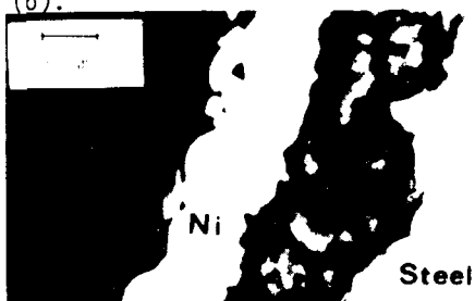
Figure 8. Cross-section of specimen 4, 2.6 mm from crack tip. SEM.
