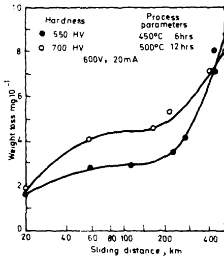
Figure 6 Wear characteristics of Iron nitrided HSLA steel
