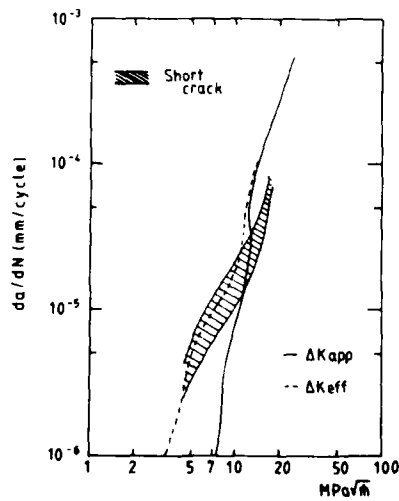
Figure 16. Small and long crack fatigue crack growth for the titanium alloy Ti 6Al 4V.
