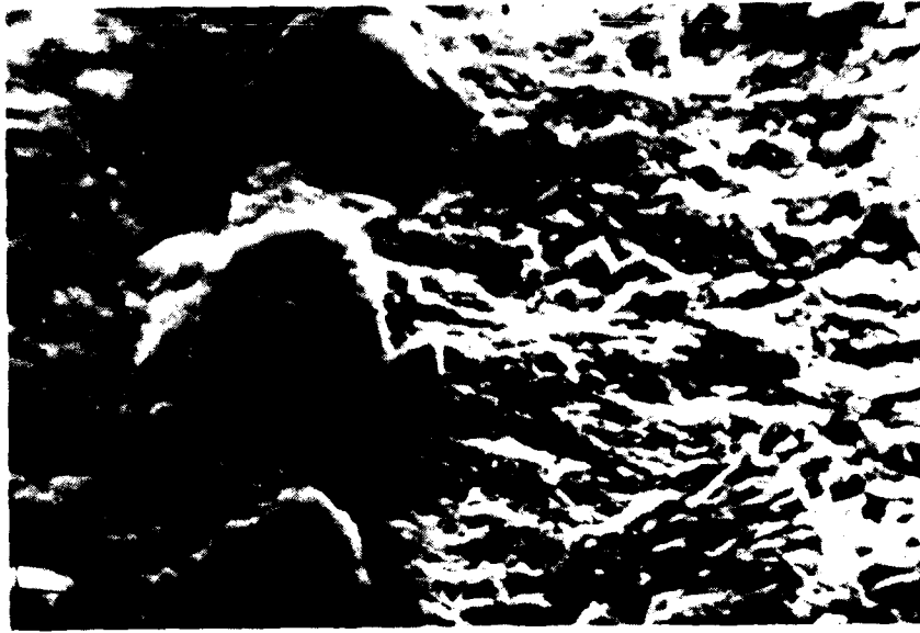
Figure 5. Nodules of oxide formed in the threshold region of a low alloy steel En 19. x 2,500
