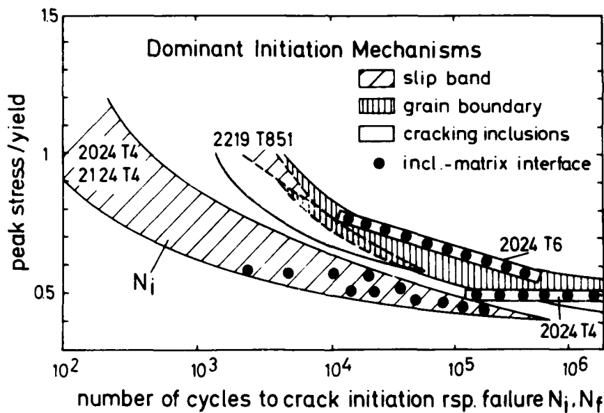
Fig. 13. Dominant crack initiation mechanisms in Al-Cu-based alloys ( R = -1 ).
