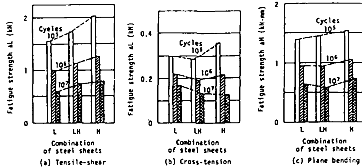
Fig. 3 Effect of combination of steel sheets on fatigue strength
