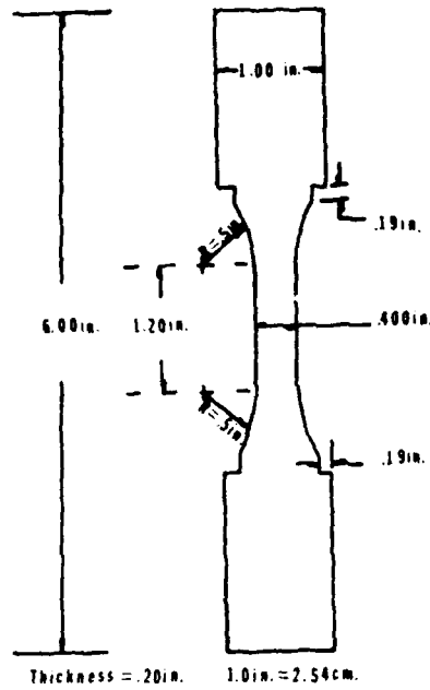
Figure 3 Small crack specimen geometry
