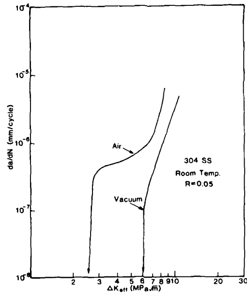
Fig. 3 da/dN vs. \Delta K plots for 304 Stainless steel for R=0.05 in air and in vacuum (6).
