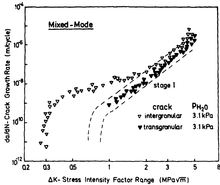
Figure 1 Crack propagation rate vs \Delta K for stage I and intergranular cracks. Scatter band after Liang et al. (8).
