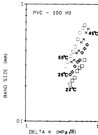
Figure 4. Discontinuous Growth Band Sizes in PVC as a Function of \Delta K and Temperature.
