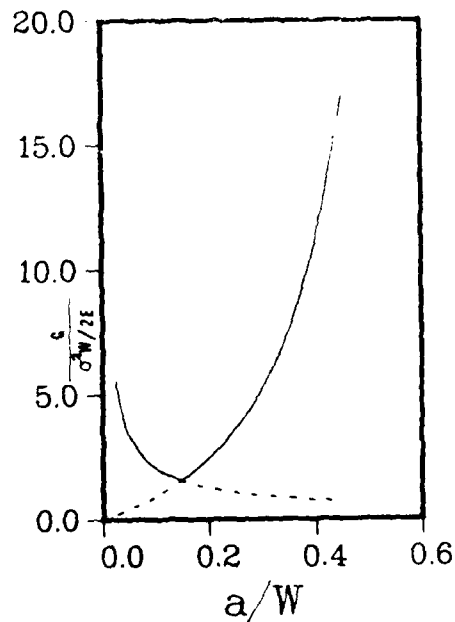
Figure 6 Strain energy release rate vs. a/W
