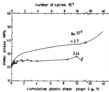
Fig. 5. Stress response of Cu-16 at.% Al single crystals fatigued at constant \gamma_{pl} . Upper scale shows the cycle numbers. Upper curve: after Abel et al (37). Lower curve: after Buchinger et al (39).
