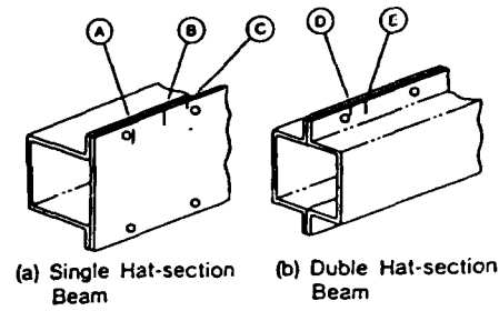
Fig.6 Fatigue Crack Mode in IN-plane Bending Fatigue Tests of Box Beam
