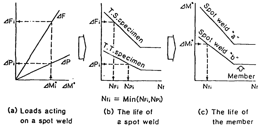
Fig.7 (a-1) The Method Based on Loads Acting to Spot Welds
