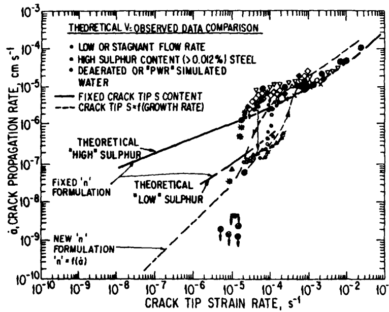
Figure 6. Comparison of predicted and observed steady state and threshold crack growth rates in deaerated water.
