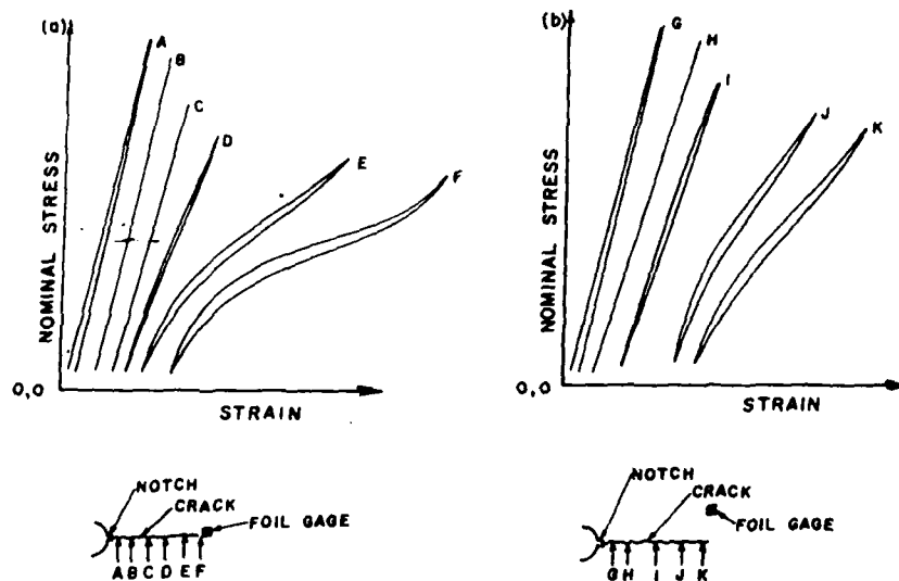
Figure 2 Typical nominal stress-strain hysteresis loops for (a) y \approx 0.020 in.
