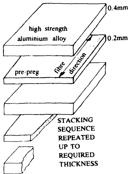
Figure 1 Laminating order of ARALL
