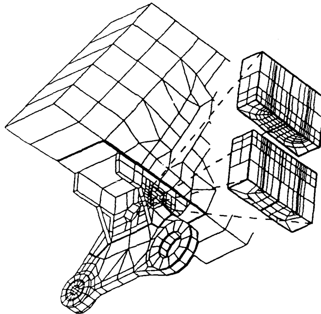
Figure 8 Structural model for stress intensity analysis of a fin attachment
