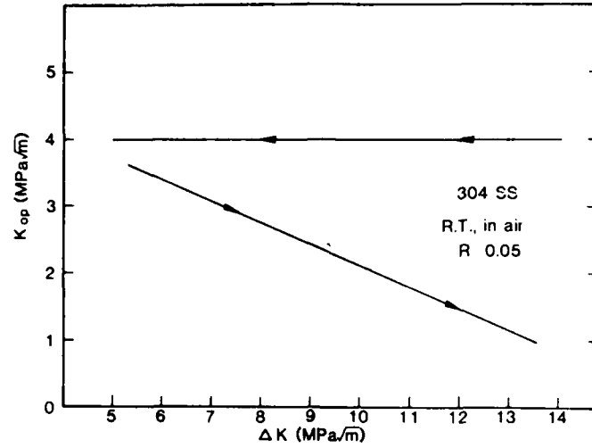
Fig. 5 Crack opening behavior of 304 stainless steel in air for \Delta K decreasing and \Delta K increasing conditions (6).
