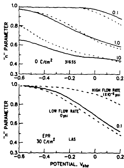
Figure 4. Comparison of predictions and empirical fits of 'n'.
