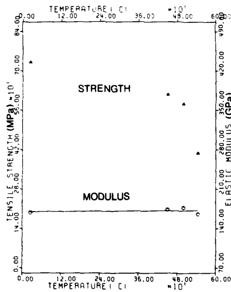
Figure 5 Tensile properties of Gr/201 Al composite as a function of exposure temperature
