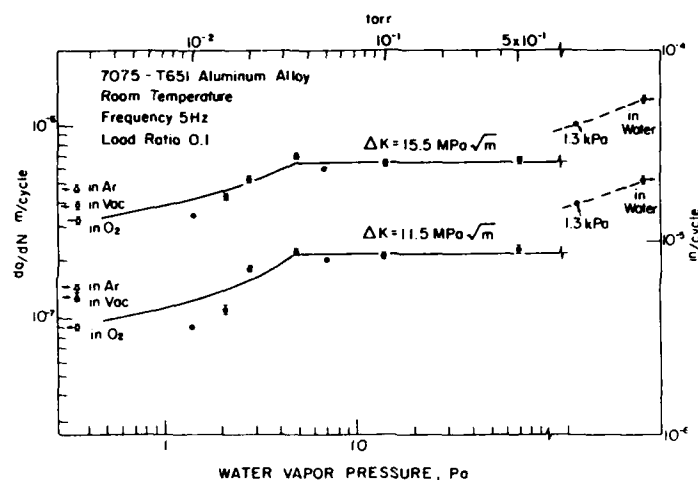
Figure 1 The influence of water vapor pressure and of other environments on fatigue crack growth in 7075-T651 (AlMgZn) alloy at room temperature. The solid lines represent predictions of a model for transport-controlled crack growth. The dashed lines indicate surface-reaction-controlled growth and reflect the influence of segregated magnesium (14)(35).
