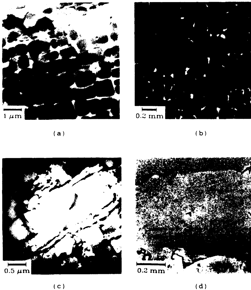
Figure 1. Initial Microstructures. (a) PWA 1480, TEM, g=\langle 200 \rangle , (b) PWA 1480 Optical Micrograph. (c) Mar-M 246 TEM, g=\langle 200 \rangle , (d) Mar-M 246 Optical Micrograph.
