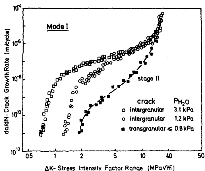
Figure 3 Crack propagation rate vs \Delta K for intergranular cracks fatigued in atmospheres with different water vapor pressures.
