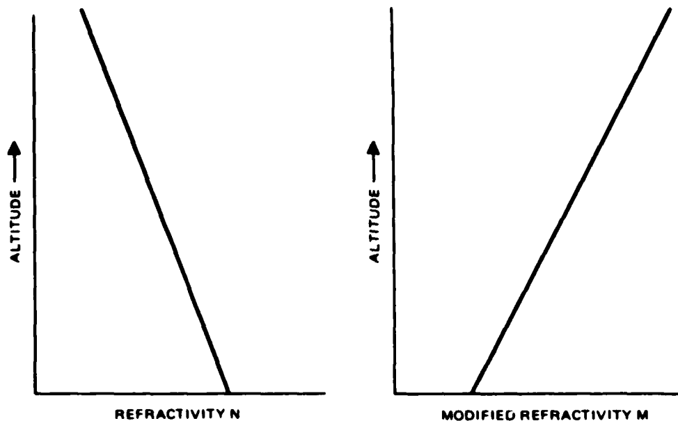
Figure 2-3. Refractivity N and modified refractivity M versus altitude for a standard atmosphere.
