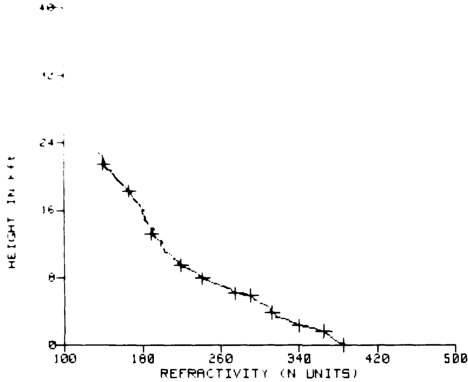
Figure 5-6. Ascent refractivity profile from figure 5-4.
