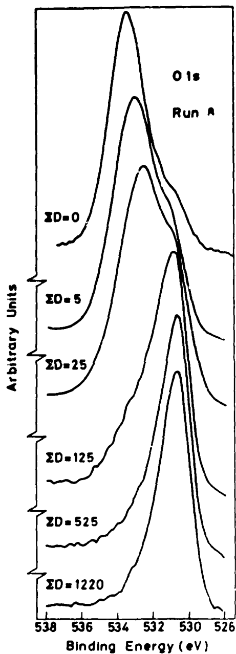
AERE R 12390 Fig. 6 Evolution of O 1s envelope as function of ion etching dose for R8, showing charge shifted peak due to either the presence of precipitated titanate on attacked surface, or a precipitated siliceous layer.
