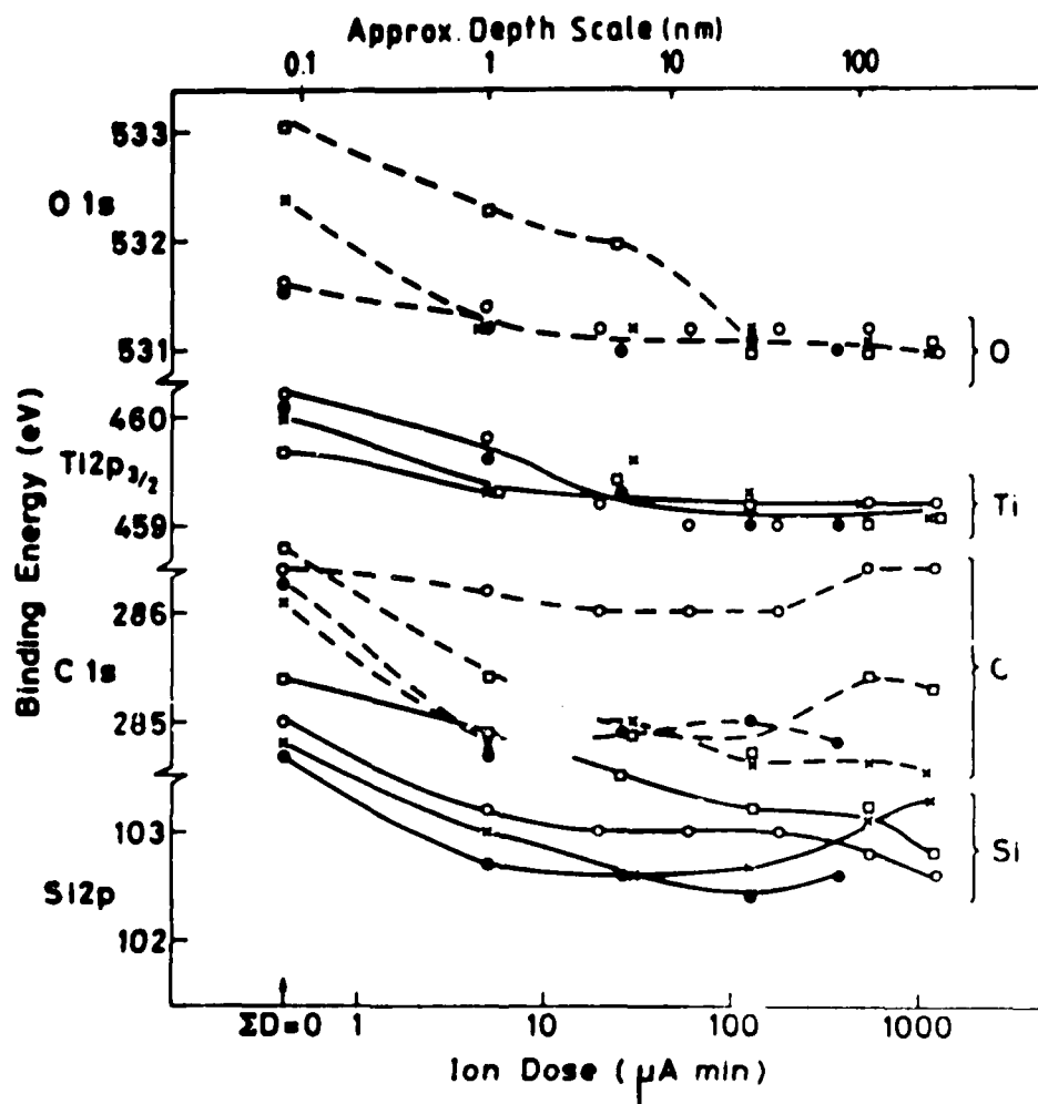
AERE R 12390 Fig 4 Binding energies of O 1s, Ti 2p 3/2 , C 1s and Si 2p electrons as functions of ion etching dose for an unetched specimen (R0) = •, (R1) = ◊, (R2) = ■, (R3) = ◊, and (R4) = x. Run conditions are listed in Table 1 and in caption for Figure 1
