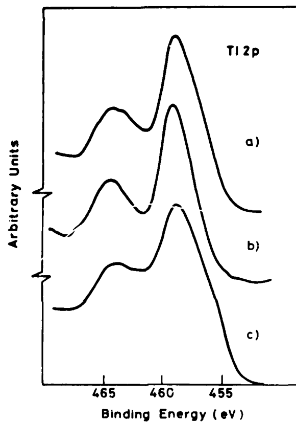
AERE R 12390 Fig. 7 Experimental Ti 2p envelopes for (a) polished unleached surface (R0), (b) 300°C for 455 hrs in DDW (R1) and (c) 175°C for 250 hrs in DDW + SiO 2 after ΣD = 100 μA mm.
