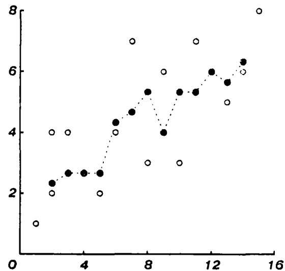
Exhibit 7-6: Smoothing
