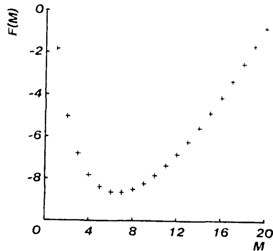
Exhibit 4-8: Minimizing F(M)
