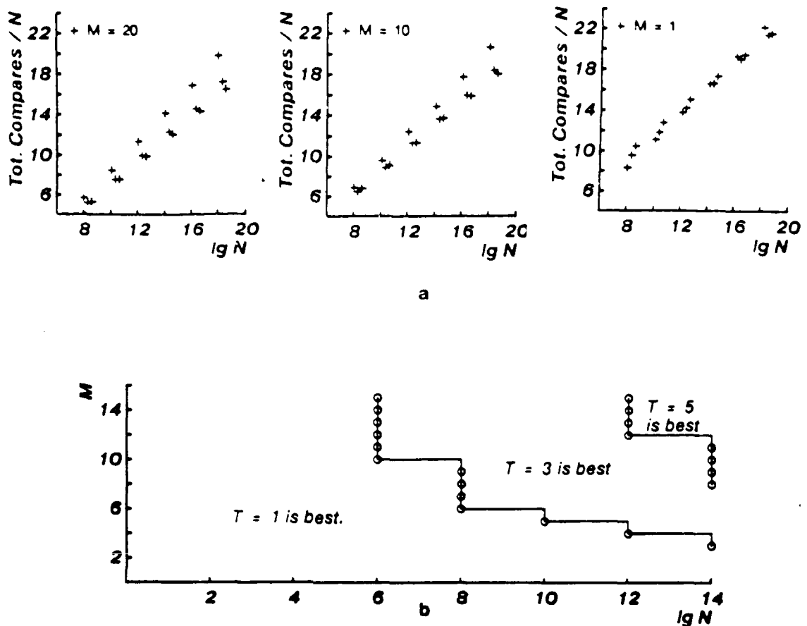
Exhibit 4-4: Total Comparisons
