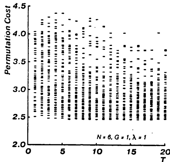
Exhibit 5-9: Permutation Distributions
