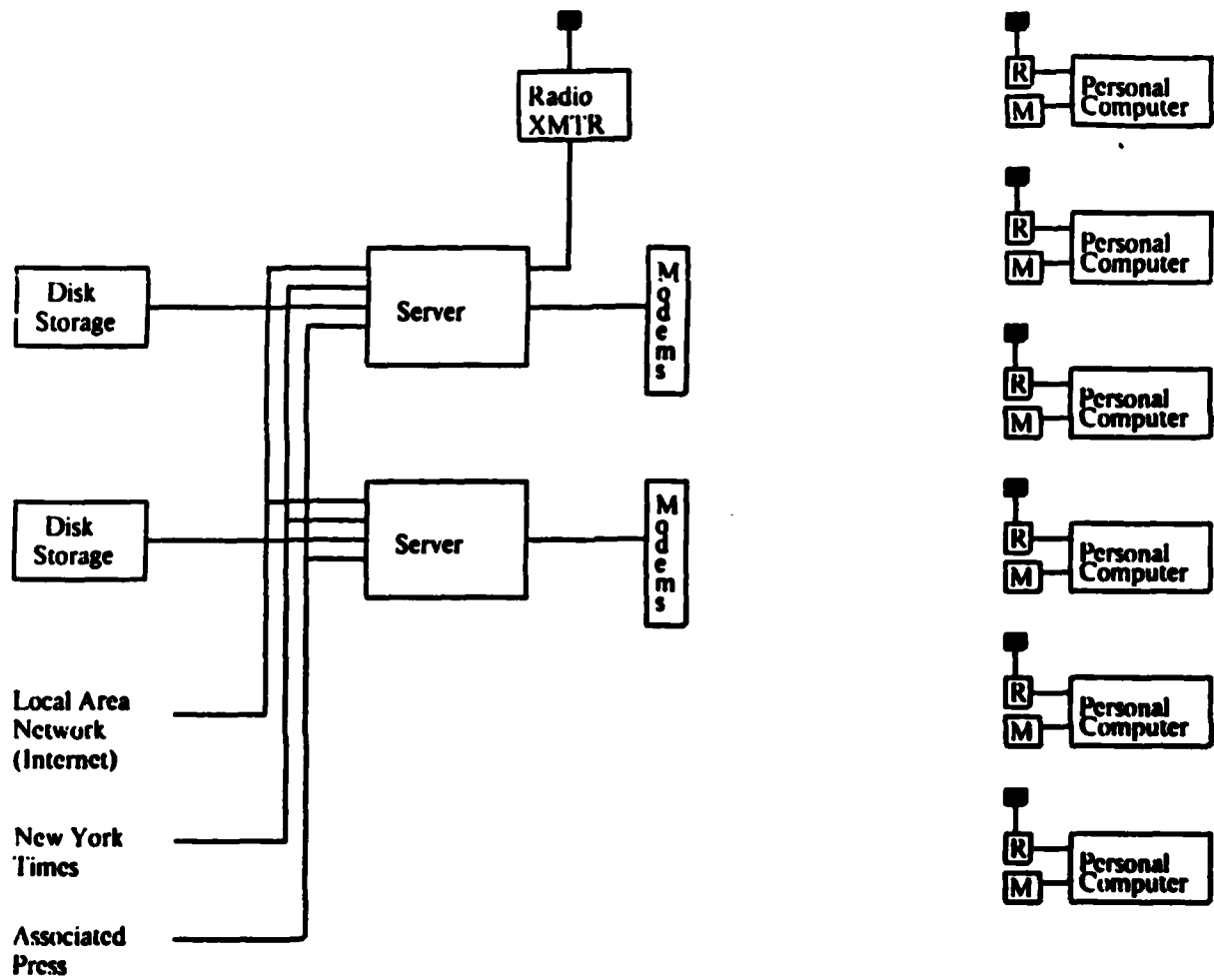
Figure 2-1: Boston CommInS System Block Diagram
