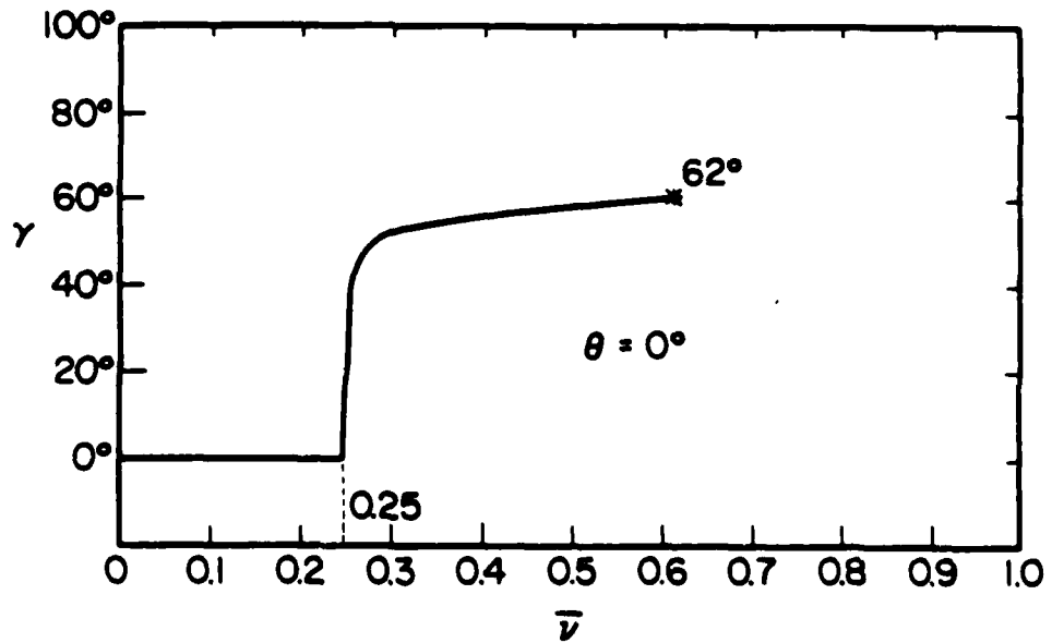
Figure 20. Meridional Position of Stress Concentration with \bar{v}
