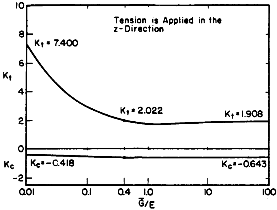
Figure 11. Variation of Stress Concentration with Modulus Ratios
