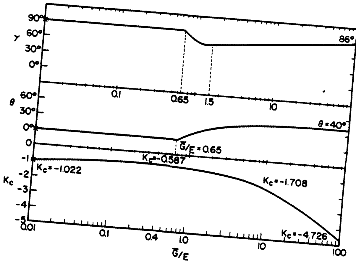
Figure 18. Compressive Stress Concentration Factor and Position versus \frac{\bar{G}}{E}
