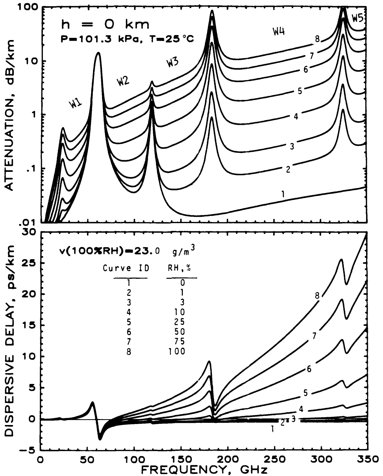
Figure 7. MPM-predicted specific values of attenuation \alpha and dispersive delay \beta at sea level height h=0 km ( P=101.3 kPa, T=25^\circ\text{C} , RH=0 to 100\% ) over the frequency range, f=1 to 350 GHz. Window ranges are marked W1 to W5.
