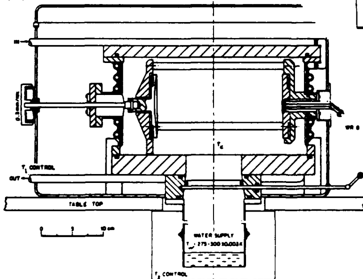
Figure 1. The high-humidity wave spectrometer: (a) photographic view, (b) schematic, (c) cell design.
