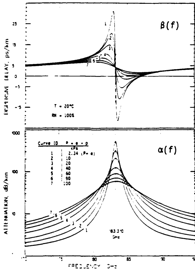
Figure 9. Pressure-broadening (AIR) example of the 183 GHz H 2 O line.
