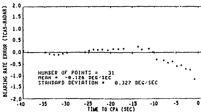
FIGURE 4.2-3. 810-KNOT, HEAD-ON ENCOUNTER (SHEET 1 OF 2)
