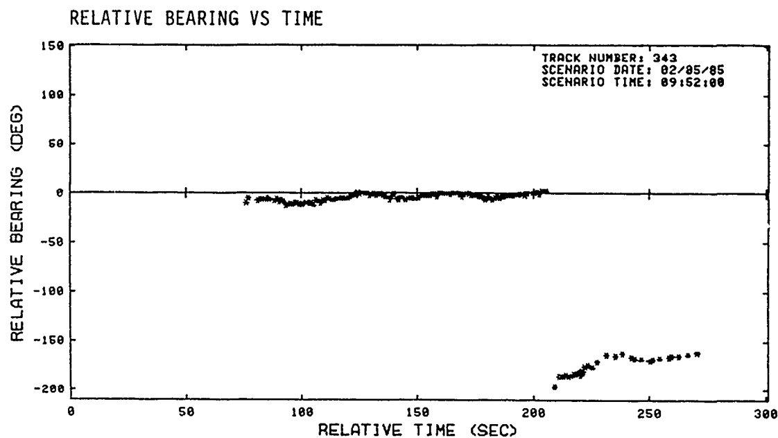
FIGURE 4.3.2-3. HEAD-ON ENCOUNTER (SHEET 1 OF 2)
