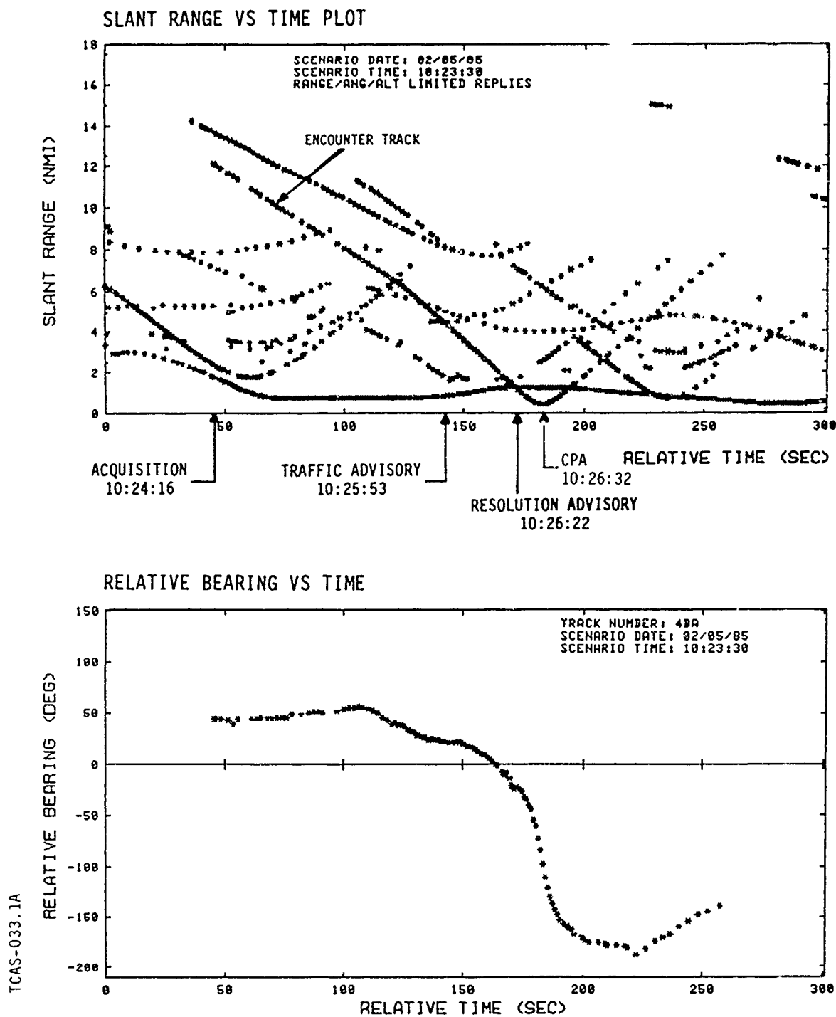
FIGURE 4.3.3-2. TARGET OF OPPORTUNITY, #2 (SHEET 1 OF 2)
