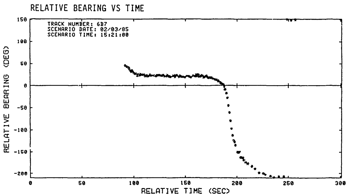
FIGURE 4.3.2-4. 45-DEGREE ENCOUNTER (SHEET 1 OF 2)
