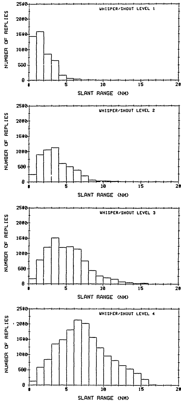
FIGURE 3.2-1. THE FOUR-LEVEL WHISPER/SHOUT USED BY ETEU#1 SHOWS EXCELLENT SEPARATION OF TARGETS IN THE L.A. BASIN
