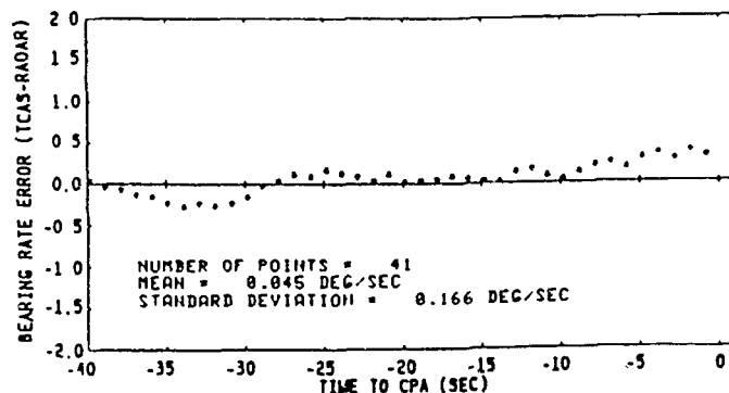
FIGURE 4.2-2. 340-KNOT, 90-DEGREE ENCOUNTER (SHEET 1 OF 2)
