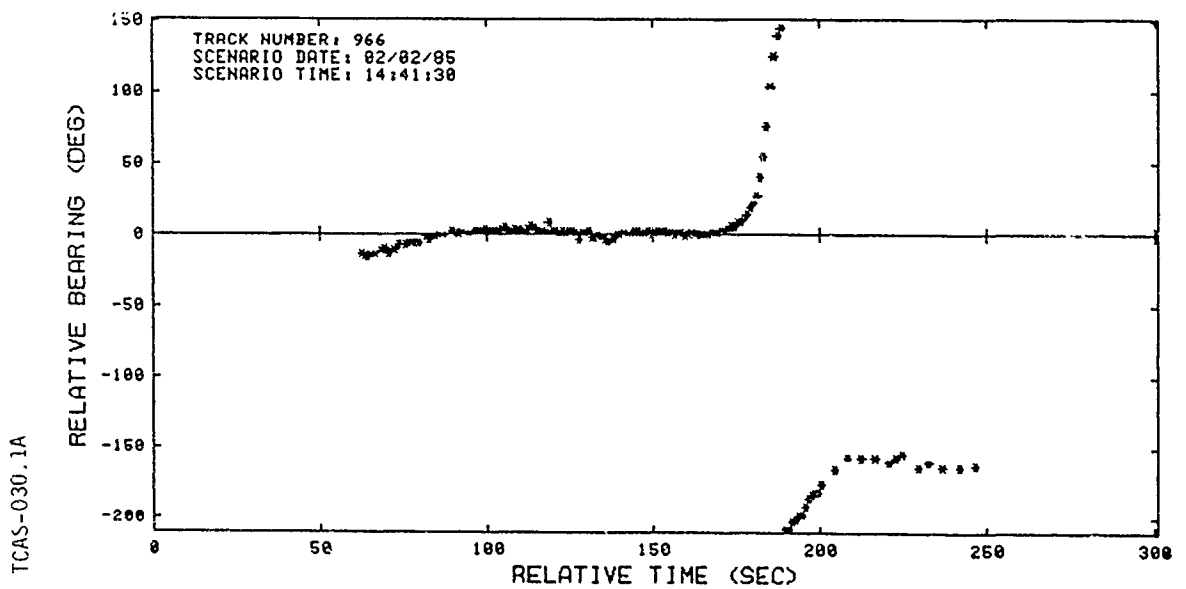
FIGURE 4.3.2-5. VERTICAL FAKEOUT (SHEET 1 OF 2)
