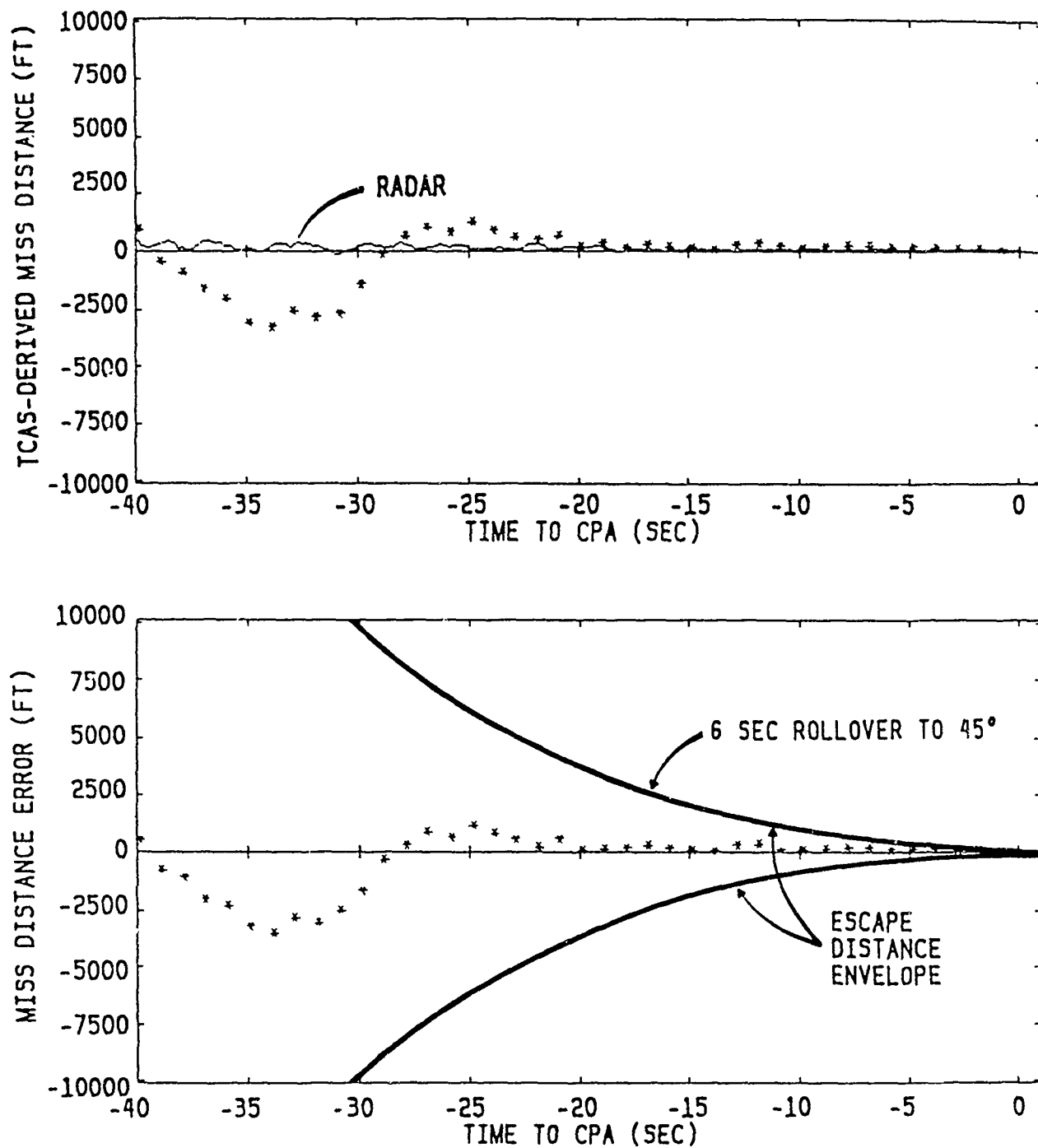
FIGURE 4.2-2. 340-KNOT, 90-DEGREE ENCOUNTER (SHEET 2 OF 2)
